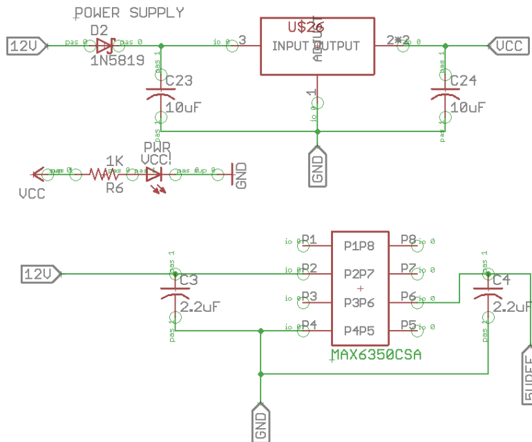
Figure B.10: 5 V linear regulator (U$26) and the voltage reference for the ADC (MAX6350CSA). The PWR LED indicates when the Power Distribution Controller is on.
