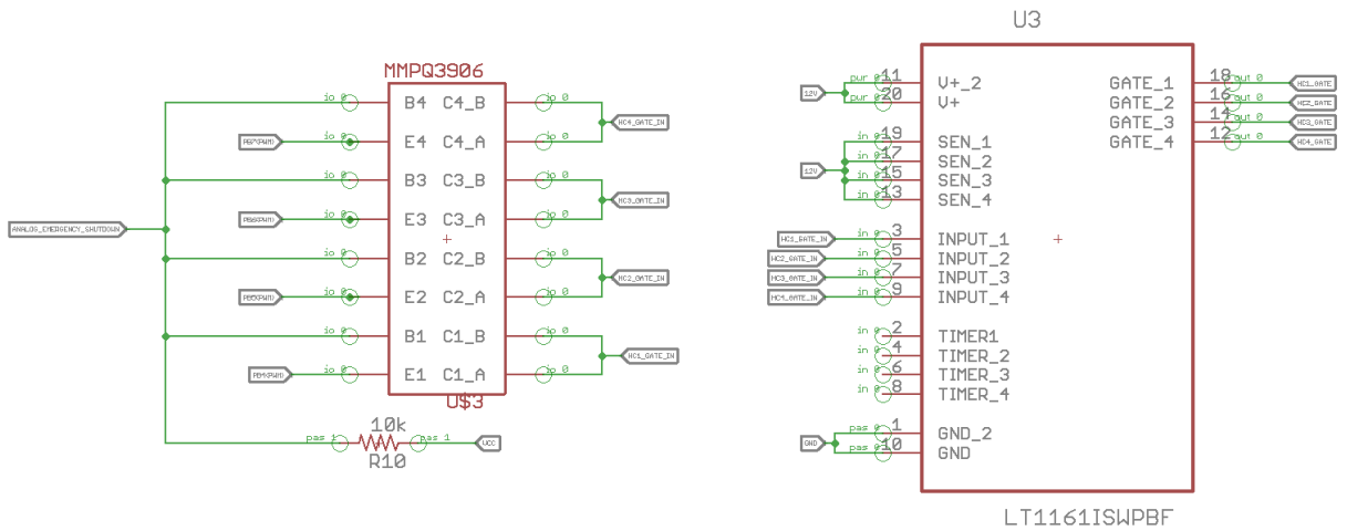
Figure B.3: Analog shut down circuitry (U$3) and gate driver for high current output (U3)
