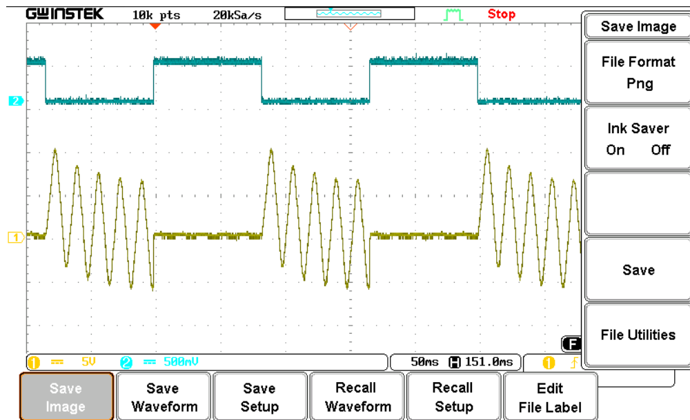
Figure 5-4. SSR Functionality Waveform
