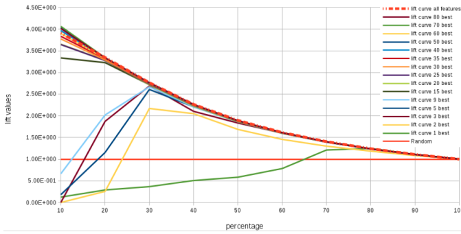
Fig. 5. Lift curves of of Extremely Randomized Forest classifiers trained with a subset of the best features
