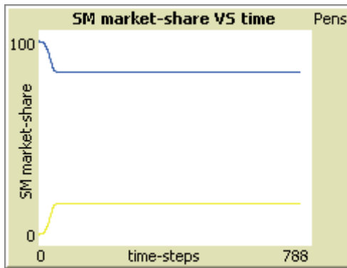
Figure 8: Scenario 3 (cooperation)
