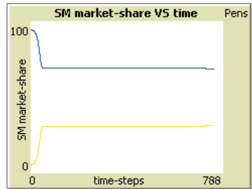
Figure 9: Scenario 4 (competition)
