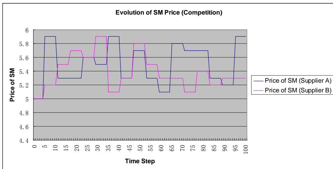
Figure 11: The Evolution of SM Price in the Competition Scenario
