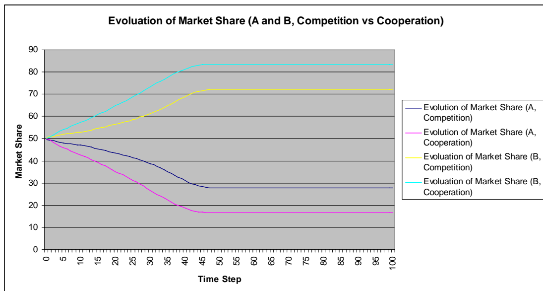
Figure 14: A Comparison between Competition (Scenario 4) and Cooperation (Scenario 3) in ES Agents Market Shares
