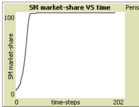
Figure 5: Scenario 1
