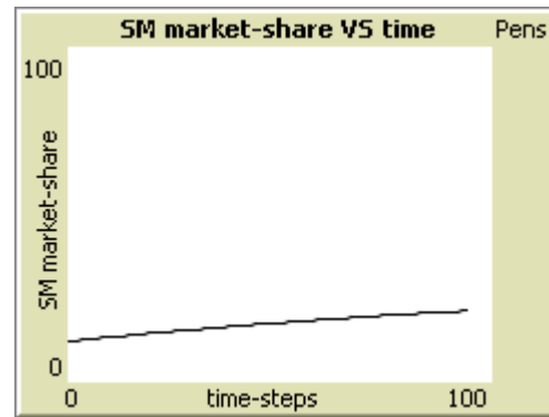
Figure 6: Scenario 2
