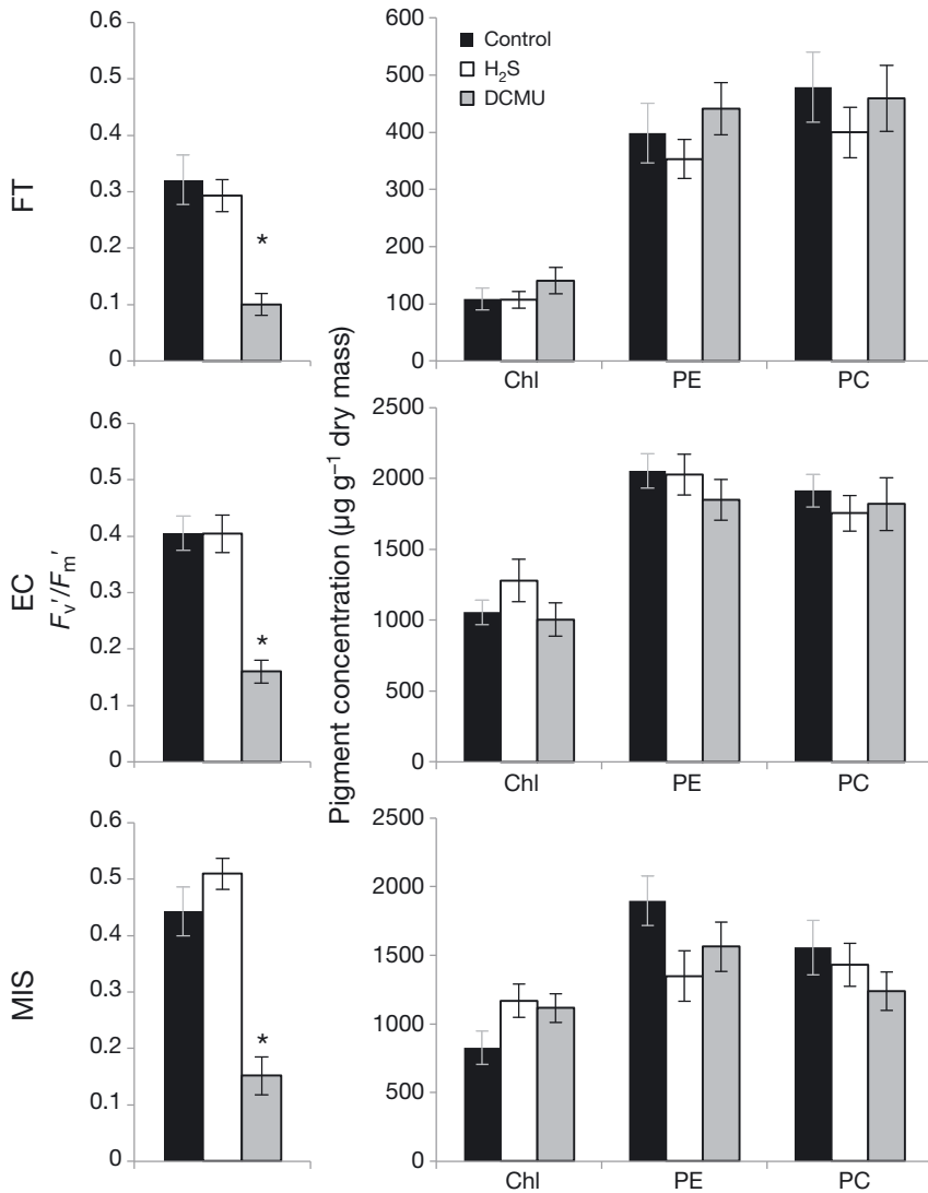
Fig. 5. Measured F_v/F_m' , chlorophyll (Chl), phycoerythrin (PE), and phycocyanin (PC) from addition of \text{H}_2\text{S} (25 to 50 \mu\text{M} ), DCMU (10 \mu\text{M} ) and a control on samples from El Cajon (EC), the Fountain (FT), and Middle Island Sink-hole (MIS). 'Control' refers to 'time 0,' or the start of the experiment. Bars: average of all measurements taken through the duration of the experiment; error bars: SE. * signifies a statistically significant group
