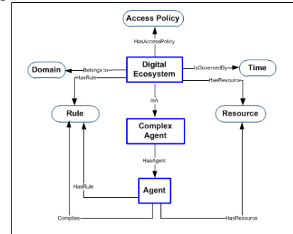
Figure 7: MAS2DES-Onto System Module
