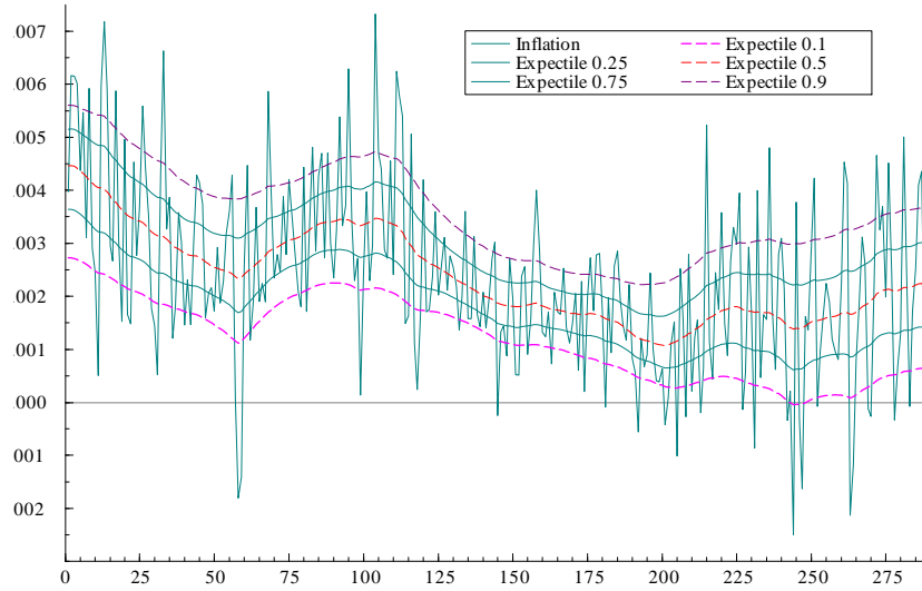
Figure 1: Time-varying RW expectiles fitted to monthly US inflation
