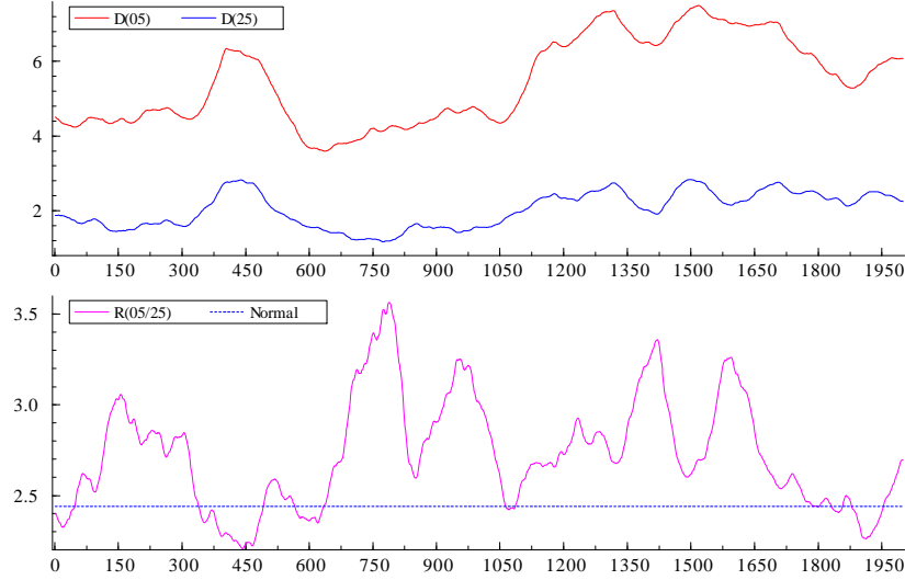
Figure 5: Interquartile, 5%-95% range and (lower graph) their ratio for GM
