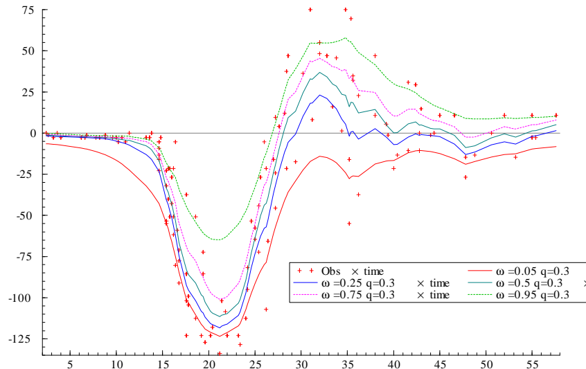
Figure 11: Time varying RW expectiles fitted to the motorcycle data. The parameter q_\mu is estimated by cross validation.
