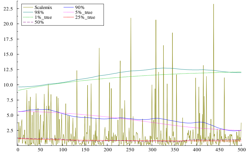
Figure 6: Absolute values of simulated series, true quantiles and random walk 98%, 90% and 50% quantiles fitted to simulated data by CV.
