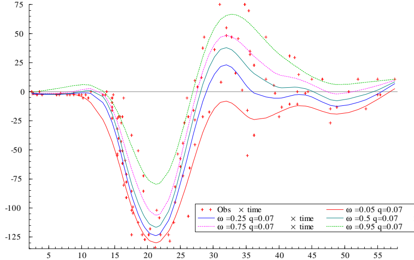
Figure 8: Cubic spline expectiles fitted to the motorcycle data. The parameter q_\mu is estimated by cross validation.
