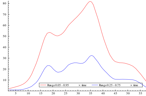
Figure 9: Motorcycle data: 75-25 and the 95-5 inter-expectile ranges.
