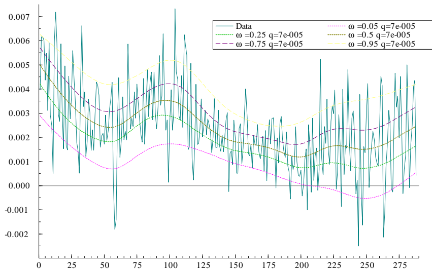
Figure 2: Time-varying cubic spline expectiles
