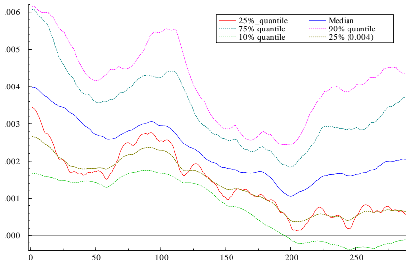
Figure 3: Inflation with two 25% quantiles
