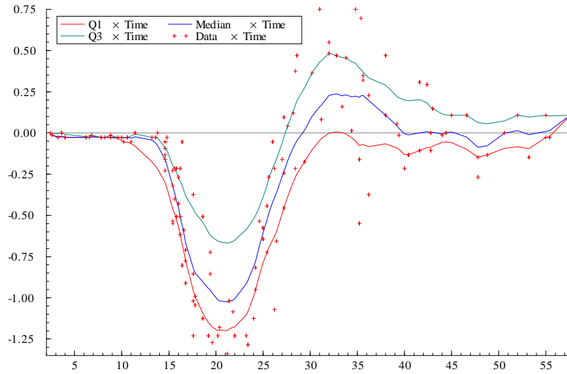
Figure 10: Quartiles and median fitted to the motorcycle data for q_\xi = 0.0625 .
