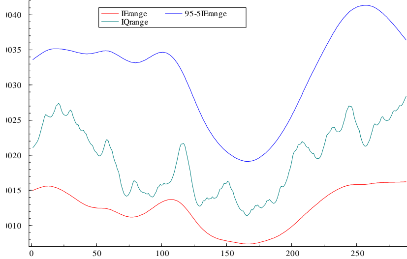
Figure 4: Inter-expectile ranges for US inflation (IRW) and IQ range (RW)
