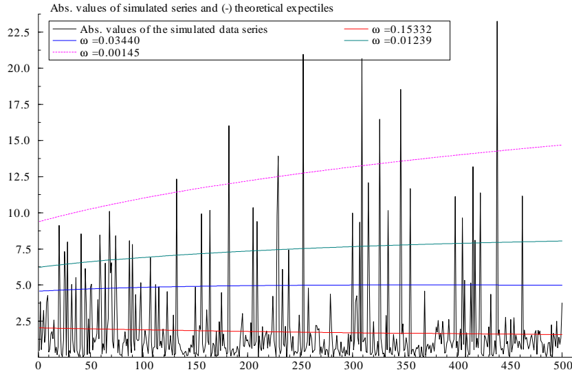
Figure 7: Absolute values of simulated series and theoretical expectiles
