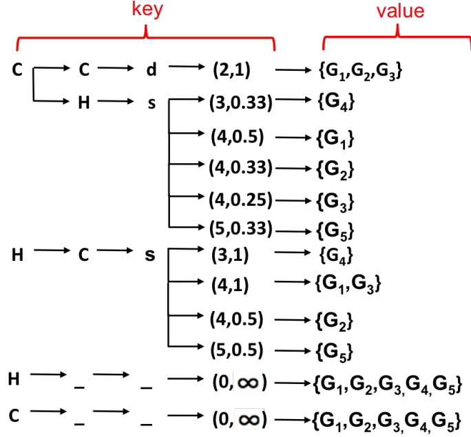
Figure 5.2: Graph-coarsening based index \mathcal{I} for graph database \mathcal{D} in Figure 5.1. The pair (c, r) denotes the collapsing edge count c and the coarsening ratio r .
