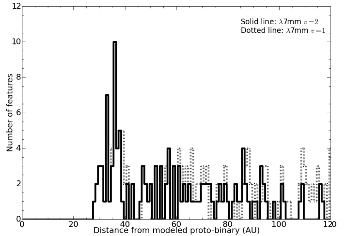
Fig. 12. Histograms showing the number of individual maser spots selected in the \lambda 7 \text{ mm } v = 1, J = 1-0 (dotted line) and v = 2, J = 1-0 (solid line) emission and their positions relative to the central object in the binary YSO pumping model (Gray et al., in prep.). The histogram bin width is 1 AU.
