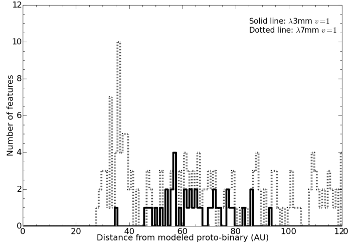
Fig. 11. Histograms showing the number of individual maser spots selected in the \lambda 3 \text{ mm } v = 1, J = 2-1 (solid line) and \lambda 7 \text{ mm } v = 1, J = 1-0 (dotted line) emission and their positions relative to the central object in the binary YSO pumping model (Gray et al., in prep.). The histogram bin width is 1 AU.
