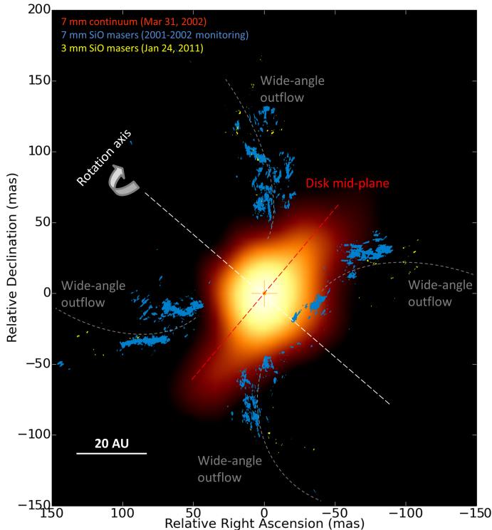
Fig. 8. Kinematic model for Source I: the bulk of the \lambda 3 mm and \lambda 7 mm ^{28}\text{SiO} maser emission is located within the four arms of a wide-angle outflow, while a dark band with no SiO emission hosts the \lambda 7 mm continuum source tracing an ionized and dusty disk (Reid et al. 2007; Plambeck & Wright 2016). The putative position of Source I is assumed to be coincident with the peak of the continuum emission.
