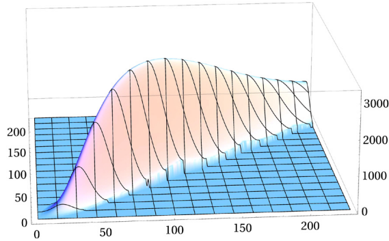
Fig. 10. Visualization of the effective transfer matrix. Horizontal axes denote spatial volume n and m , respectively, and vertical axis denote value of matrix elements \langle n|M|m \rangle .
