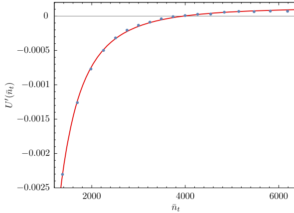
Fig. 7. First derivative of the potential extracted from the classical trajectory (blue dots) and a power-law fit U'(n) = \lambda + \text{const} \times n^{\gamma-1} , \gamma \approx -1.78 \pm 0.1 .
