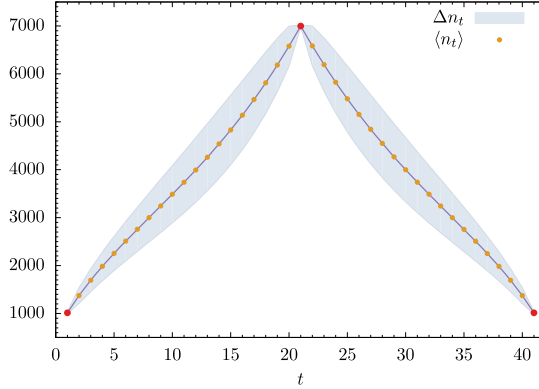
Fig. 3. Average volume profile \langle n_t \rangle measured for bare coupling constants \kappa_0 = 2.2 , \kappa_4 = 0.9225 , \Delta = 0.6 and time period T = 40 . Red dots denote time slices with fixed volume, \hat{n}_1 = 1000 and \hat{n}_h = 7000 , h = T/2 + 1 . (For interpretation of the references to color in this figure legend, the reader is referred to the web version of this article.)
