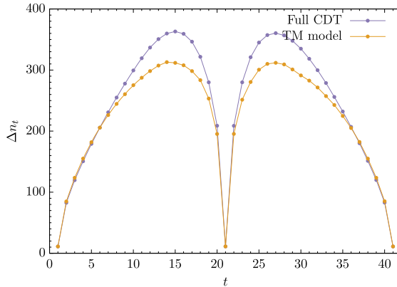
Fig. 15. Amplitude of fluctuations of the spatial volume \Delta n_t obtained for the full CDT model and using the effective transfer matrix model.
