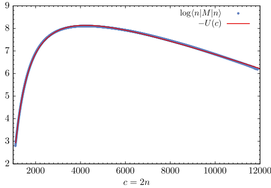
Fig. 13. Logarithm of the transfer matrix diagonal \langle n|M|n\rangle measured via the normalization factor of the Gaussian fit of the cross-diagonals (blue dots) and power-law (red line) fit of the potential U(c) . (For interpretation of the references to color in this figure legend, the reader is referred to the web version of this article.)
