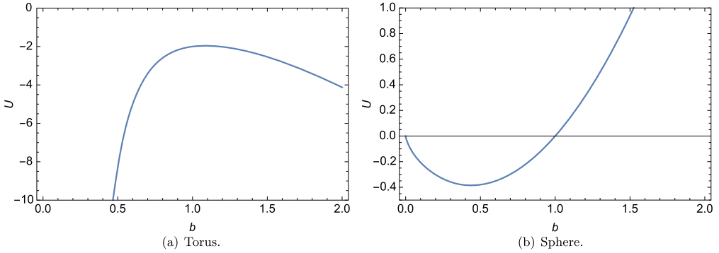
Fig. 8. The effective potential U[b] for the sphere and torus cases.
