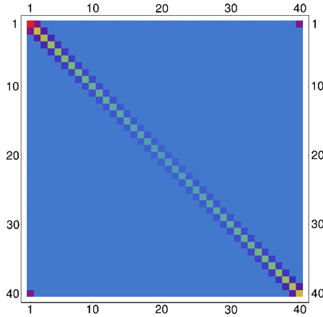
Fig. 4. Density plot of the covariance matrix inverse, P = C^{-1} . The tri-diagonal structure is well visible. The entries of P outside the tri-diagonal are zero up to numerical noise.
