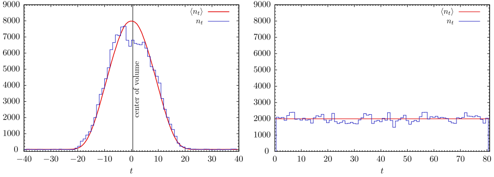
Fig. 2. The average (red) and typical (blue) volume profiles for spherical spatial topology (left figure) and for toroidal spatial topology (right figure) in the so-called de Sitter phase ( C_{dS} ). In both cases the time direction has length 80 (in lattice units) with periodic boundary conditions. In the case of spherical spatial topology the “effective” time extent is approximately 40 lattice units and scales as N^{1/4} , N being the total four-volume of the universe, while n_t scales as N^{3/4} . This is in contrast to the case of toroidal spatial topology where n_t is macroscopic for all t and scales as N/T , T being the time extent. (For interpretation of the references to color in this figure legend, the reader is referred to the web version of this article.)
