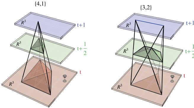
Fig. 1. Visualization of fundamental building blocks in four-dimensional CDT. A (4, 1) simplex (left) has four vertices at (discrete) proper time t (forming a tetrahedron) and one vertex at time t + 1 . A (3, 2) simplex (right) has three vertices at time t and two at t + 1 . Cauchy surfaces for non-integer t are built from a combination of tetrahedra (obtained by slicing (4, 1) simplices with hyperplanes of constant time) and triangular prisms (from (3, 2) simplices).
