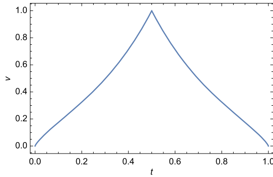
Fig. 9. The classical trajectory interpolating between zero initial volume and some intermediate volume.
