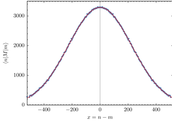
Fig. 11. Cross-diagonal of the transfer matrix for c = n + m = 4000 . It matches a Gaussian function \mathcal{N}(c) e^{-x^2/f(c)} .
