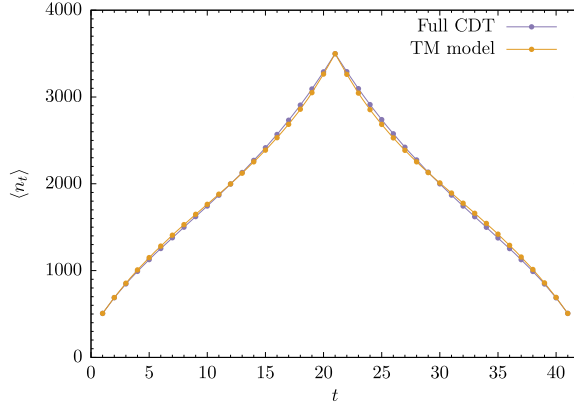
Fig. 14. Average volume profile \langle n_t \rangle obtained for the full CDT model and using the effective transfer matrix model.
