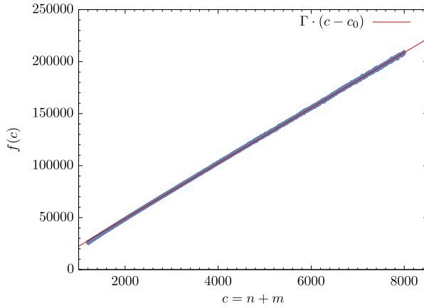
Fig. 12. Plot of the kinetic term f(c) extracted by fitting a Gaussian function \mathcal{N}(c) e^{-x^2/f(c)} to \langle n = \frac{c+x}{2} | M | m = \frac{c-x}{2} \rangle matrix elements for various values of c = n + m (blue dots) and a linear fit (red line). (For interpretation of the references to color in this figure legend, the reader is referred to the web version of this article.)
