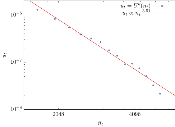
Fig. 6. Log–log plot of the potential coefficients u_t as a function of \langle n_t \rangle .
