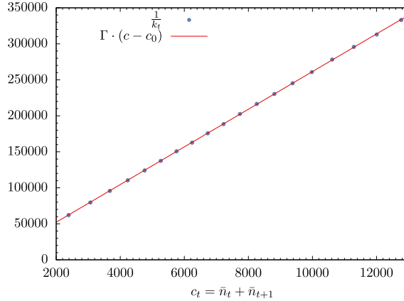
Fig. 5. Inverse of the kinetic term k_t = -\frac{1}{2}P_{tt+1} as a function of volume c_t = \langle n_t \rangle + \langle n_{t+1} \rangle . A linear fit \Gamma \cdot (c - c_0) is very accurate. (For interpretation of the references to color in this figure, the reader is referred to the web version of this article.)
