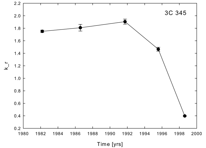
Figure 6. 3C 345: time evolution of k_r values.
