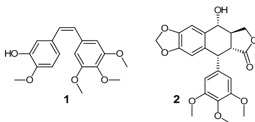
Figure 1. Structures of Combretastatin A4 (CA-4, 1) and podophyllotoxin 2.
