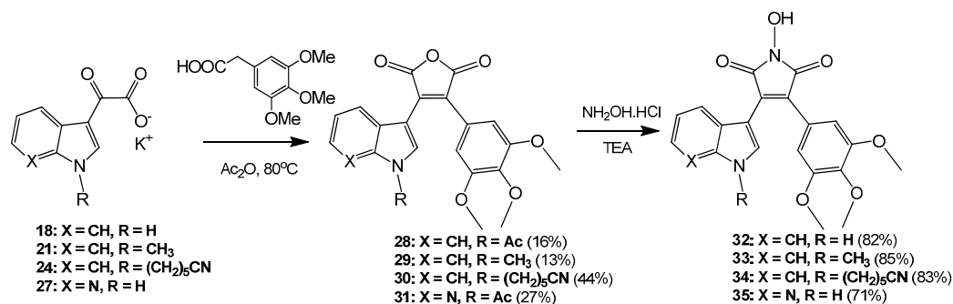
Scheme 3. Route to 3,4-diaryl-1-hydroxymaleimides 32–35 .
