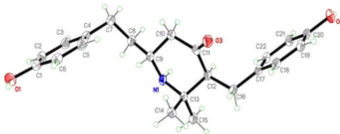
Figure 1 The ORTEP view of pellacalyxin( 1 ) obtained by X-ray crystallography.
