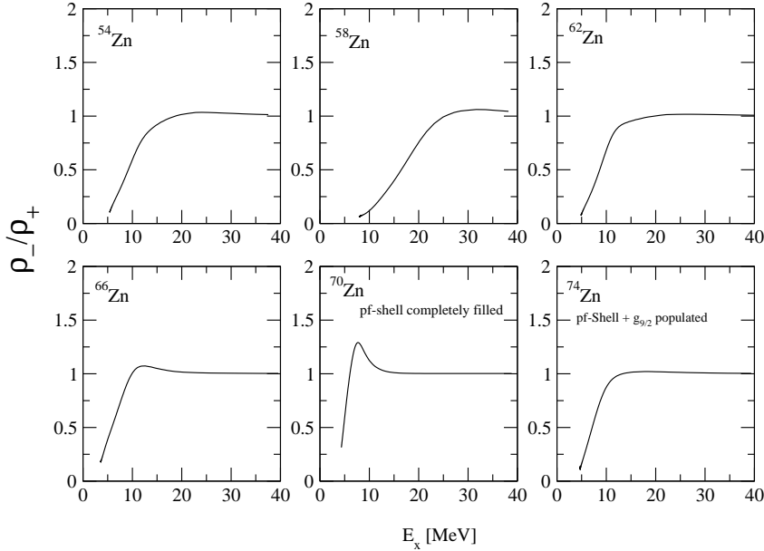
Figure 2. Evolution of the odd- to even-parity ratio within the Zn-chain.
