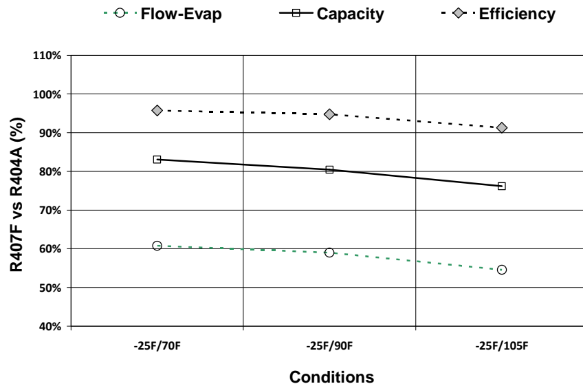
Figure 5. Standard Compressor Calorimeter tests.
