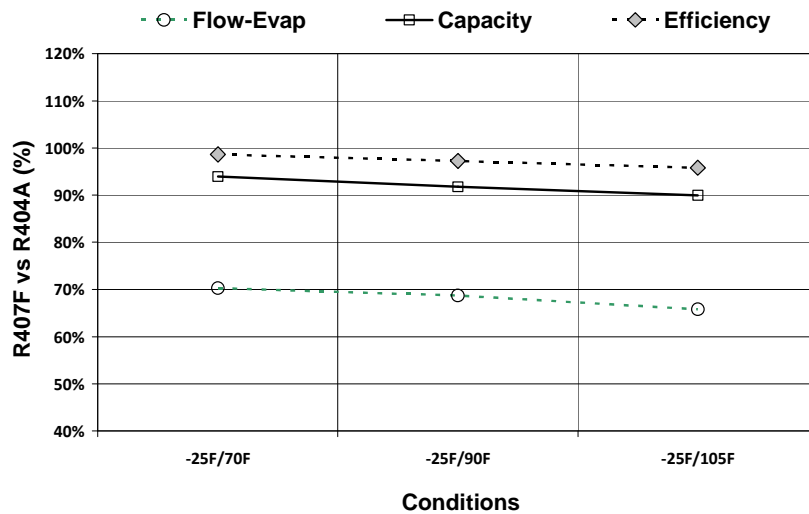
Figure 6. Modified test using average pressures for evaporating and condensing processes.
