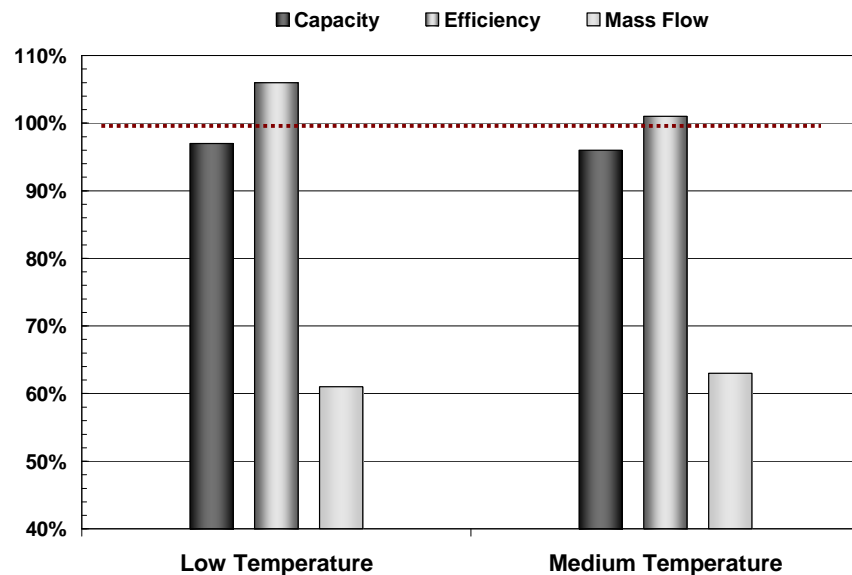
Figure 4. Lowest GWP Option L-40 (relative to R-404A).
