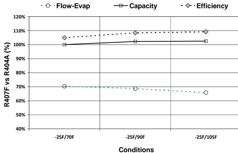
Figure 7. Combined effect of using average pressures and 10°F superheat at evaporator outlet.
