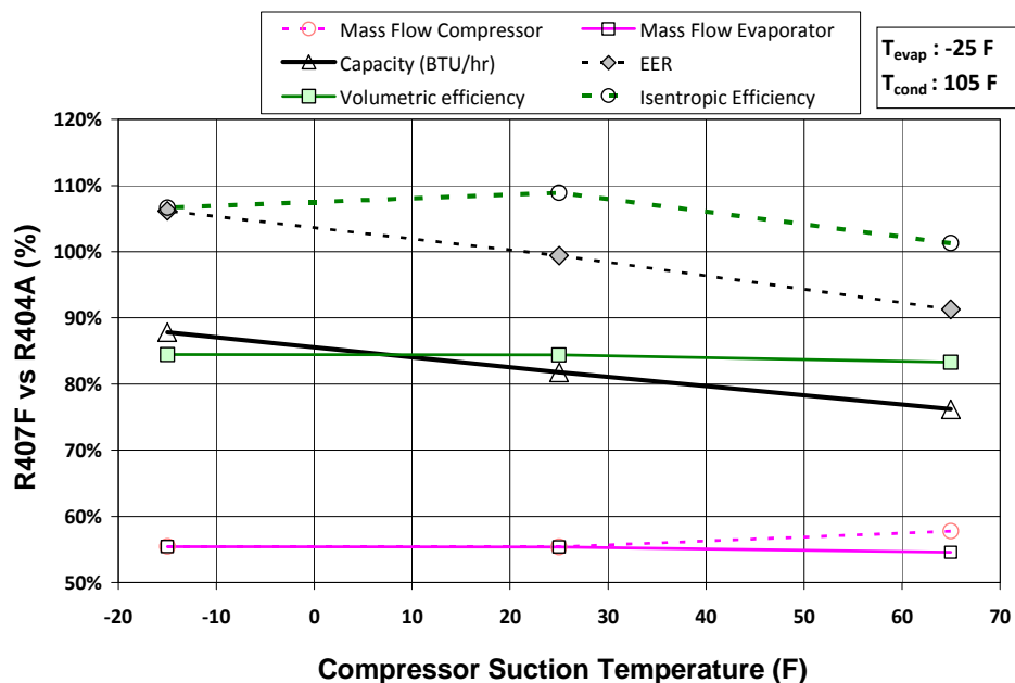
Figure 8. Effect of suction temperature on compressor efficiency.
