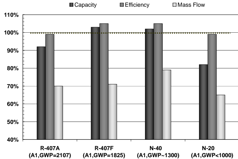
Figure 3. Medium Temperature Tests (relative to R-404A).
