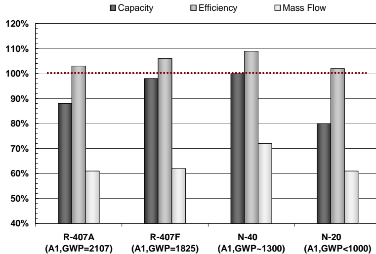
Figure 1. Low Temperature Performance (relative to R-404A).
