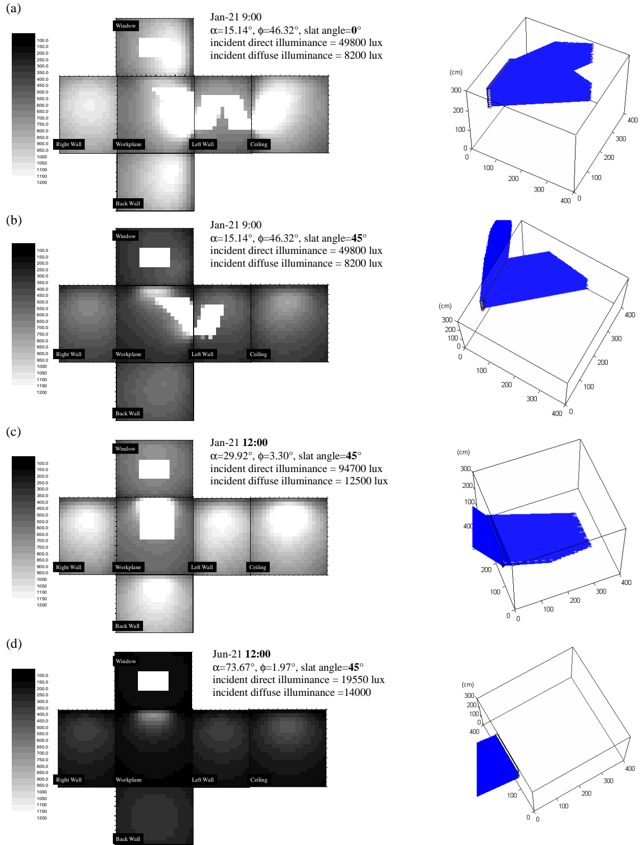
Figure 9: (a) Illuminance distribution contours on Jan-21 9:00 with 0^\circ slat angle; (b) Jan-21 9:00 with 45^\circ slat angle; (c) Jan-21 12:00 with 45^\circ slat angle; (d) Jun-21 12:00 with 45^\circ slat angle;
