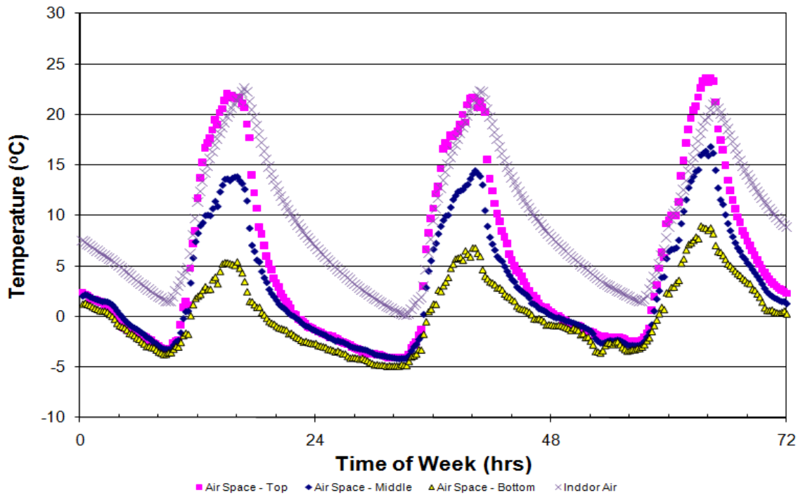
Figure 7 Winter facade cavity temperatures
