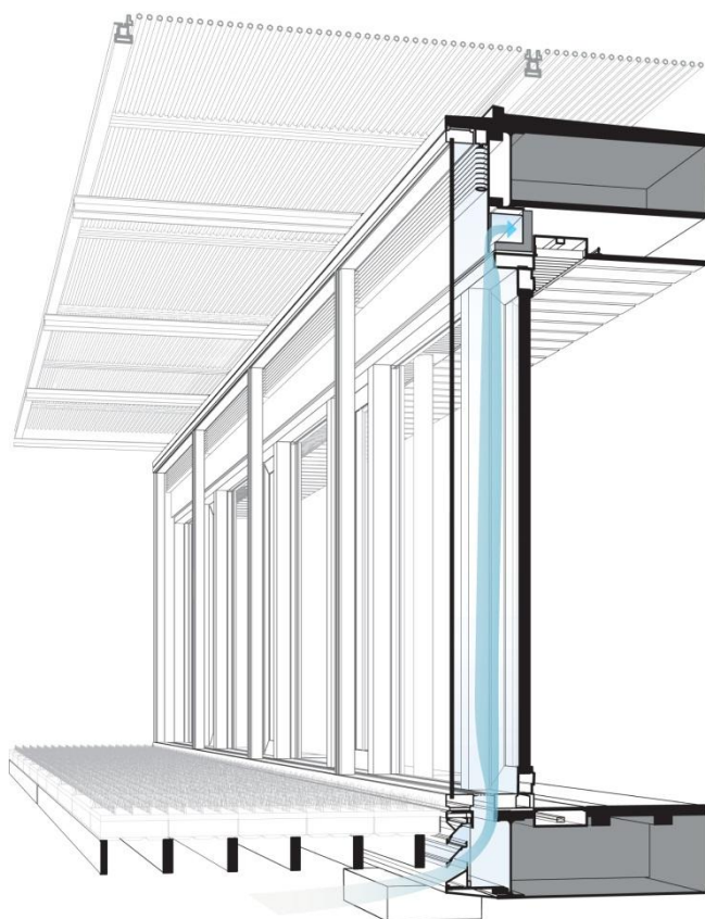
Figure 5. Section through the south façade from BIM model
