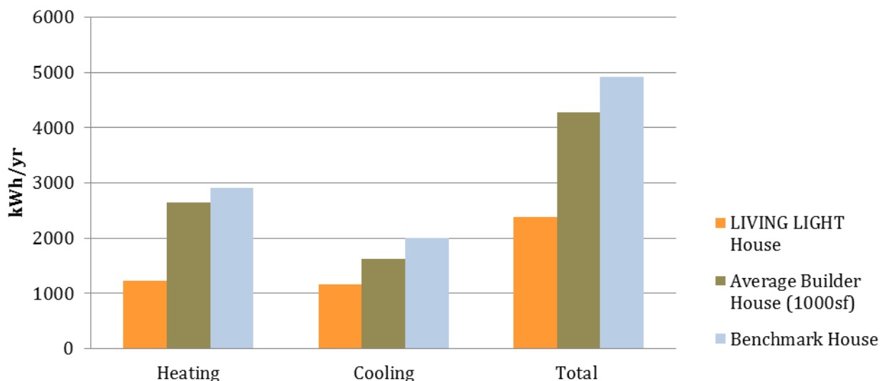
Figure 13. Heating and cooling comparison
