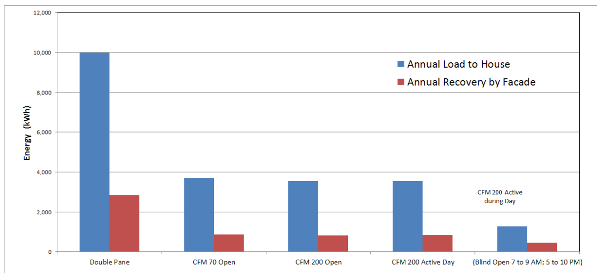
Figure 8. Optimal façade configurations and energy balance
