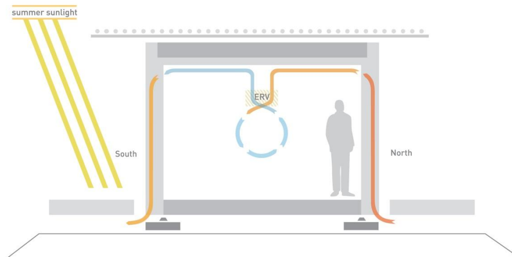
Figure 11. Summer cooling mode showing ventilation through the double façade.
