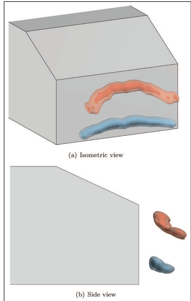
Figure 5. Three-dimensional representations of spanwise \Gamma_1 criterion. Red represents a positive rotation (A region), blue represents a negative rotation (B region). Colours are consistent with Figure 4.
