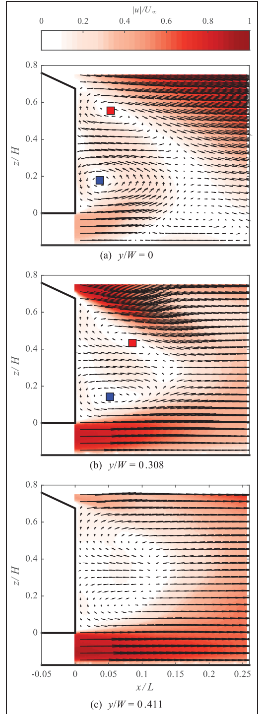
Figure 3. Flow in the xz planes behind the Ahmed model with velocity vectors overlaid onto contours of total velocity magnitude. Only one in one hundred velocity vectors are shown for clarity. The red and blue points indicate the core of the A and B vortical structures respectively, found as the maximum and minimum of \Gamma_1 respectively.
