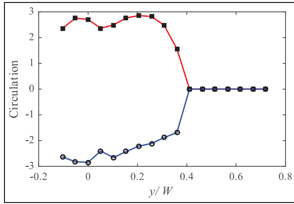
Figure 6. The spanwise circulation bound in the A (red, squares) and B (blue, circles) vortical structures against spanwise position. Circulation is non-dimensionalised with the free-stream velocity and the square-root of the frontal area.
