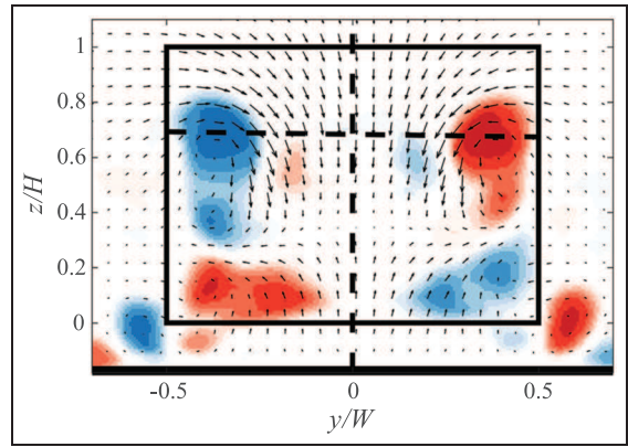
Figure 8. Cross-stream PIV plane 0.1L behind the high-drag Ahmed model showing the trailing legs of the B vortex as well as the combined A and C-pillar vortices. One in 64 vectors are displayed for clarity. Filled contours are \Gamma_2 ranging from -1 in blue (clockwise rotation) to 1 in red (counter-clockwise rotation). Source: reproduced with permission from Monash University, 2016. 20
