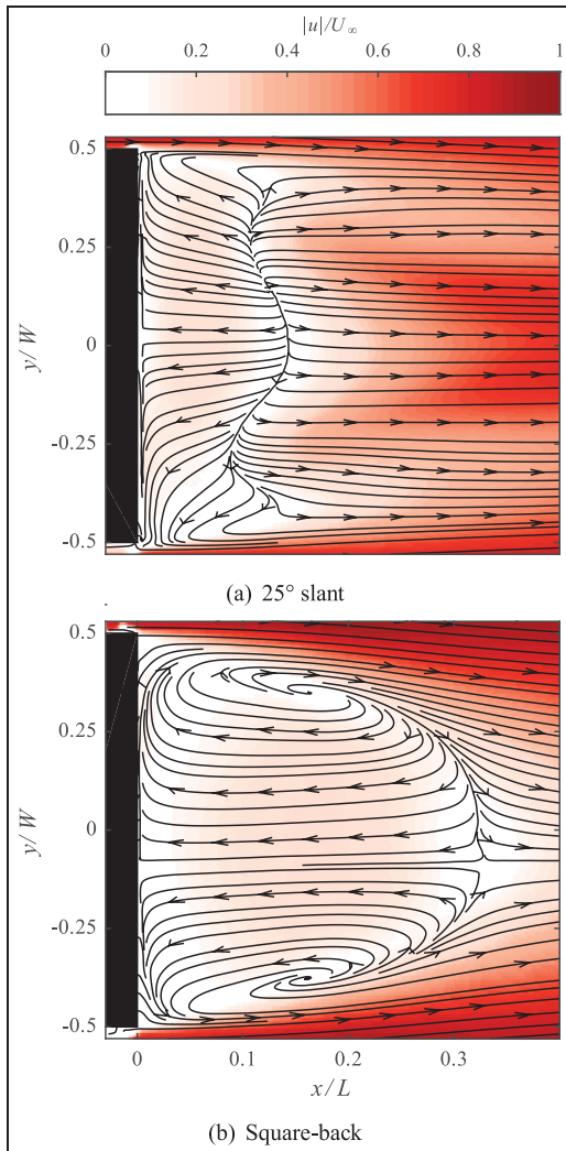
Figure 7. (a) Flow in the xy plane at z/H=0.369 with velocity streamlines overlaid onto filled contours of total velocity. (b) Flow behind the square-back Ahmed geometry at the mid-height plane clearly showing the vertical legs of the toroidal vortex. Streamlines are used to indicate the local flow direction only.
