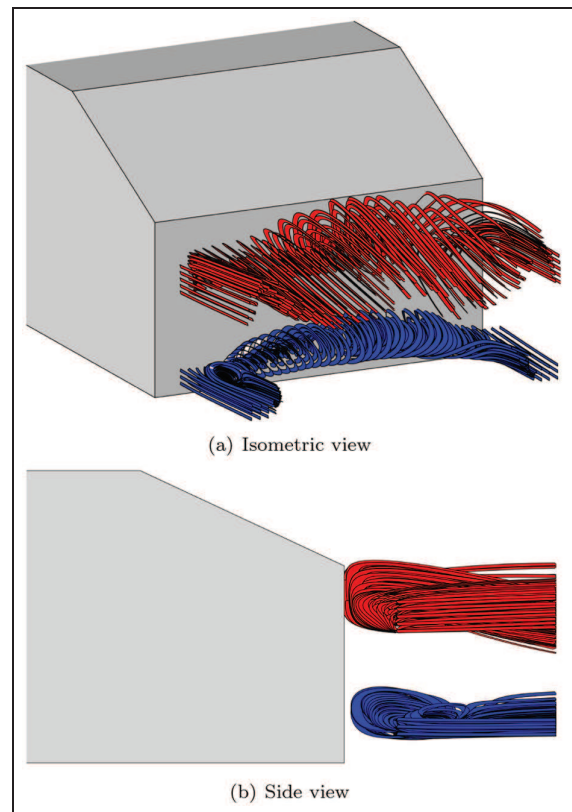
Figure 9. Streamribbons with seed points in the A (red) and B (blue) regions. Especially in the B region, spanwise flow is clearly evident until the edge of the body, where the streamribbons are tilted in the streamwise direction.
