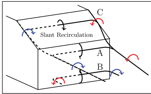
Figure 10. Vortex structure schematic in the wake of the Ahmed body, with lines indicating the location of the vortex cores. The structure is dashed for y/W < 0 and solid for y/W > 0 . Spanwise rotation is indicated by black arrows and streamwise rotation is indicated by red or blue arrows for positive or negative rotation, respectively.
