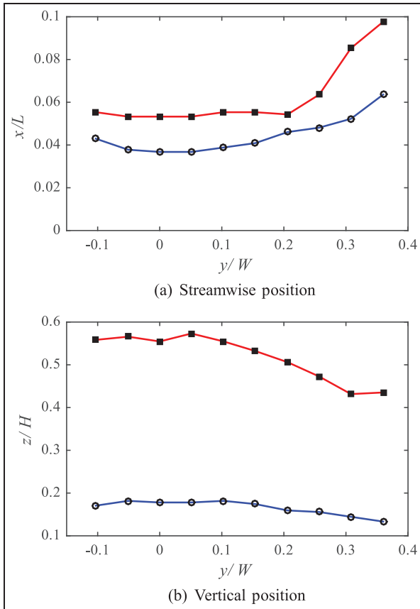
Figure 4. Core location of the A (red, squares) and B (blue, circles) vortical structures against spanwise position.
