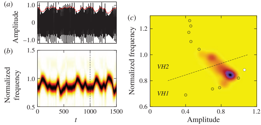
FIGURE 17. (Colour online) Time–frequency analysis of the cross-flow displacement in the VH1 – VH2 transition region, (\beta, U^*) = (0.3, 9) : (a) selected time series of \zeta_y , (b) spectrogram and (c) histogram of the instantaneous frequency ratio ( f_y^{i*} ) and amplitude ( \zeta_y^i ). In (a), a red dashed line indicates the instantaneous amplitude of the displacement signal. The spectrogram and histogram are normalized by the magnitude of the largest peak. In the spectrogram, a vertical dashed line indicates the beginning of the time interval considered in figure 18. In the histogram, symbols indicate the values of (\zeta_y^m, f_y^*) obtained for \beta = 0.3 and all U^* and the case under study, U^* = 9 , is denoted by a white symbol; a dashed line delimitates the regions associated with regimes VH1 and VH2 .
