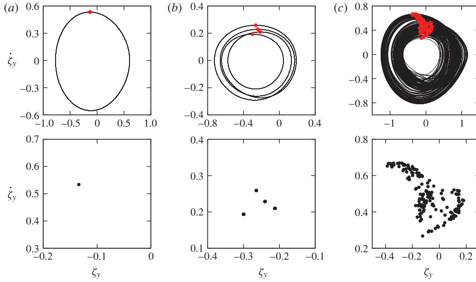
FIGURE 16. (Colour online) Periodicity of the cross-flow displacement in the high-shear region: phase portrait (upper row) and Poincaré map (lower row) of \zeta_y for \beta = 0.3 and (a) U^* = 6 (regime VH1 ), (b) U^* = 12 (regime VH2 ) and (c) U^* = 9 (transition region). In each phase portrait, red dots indicate the points plotted in the Poincaré map.
