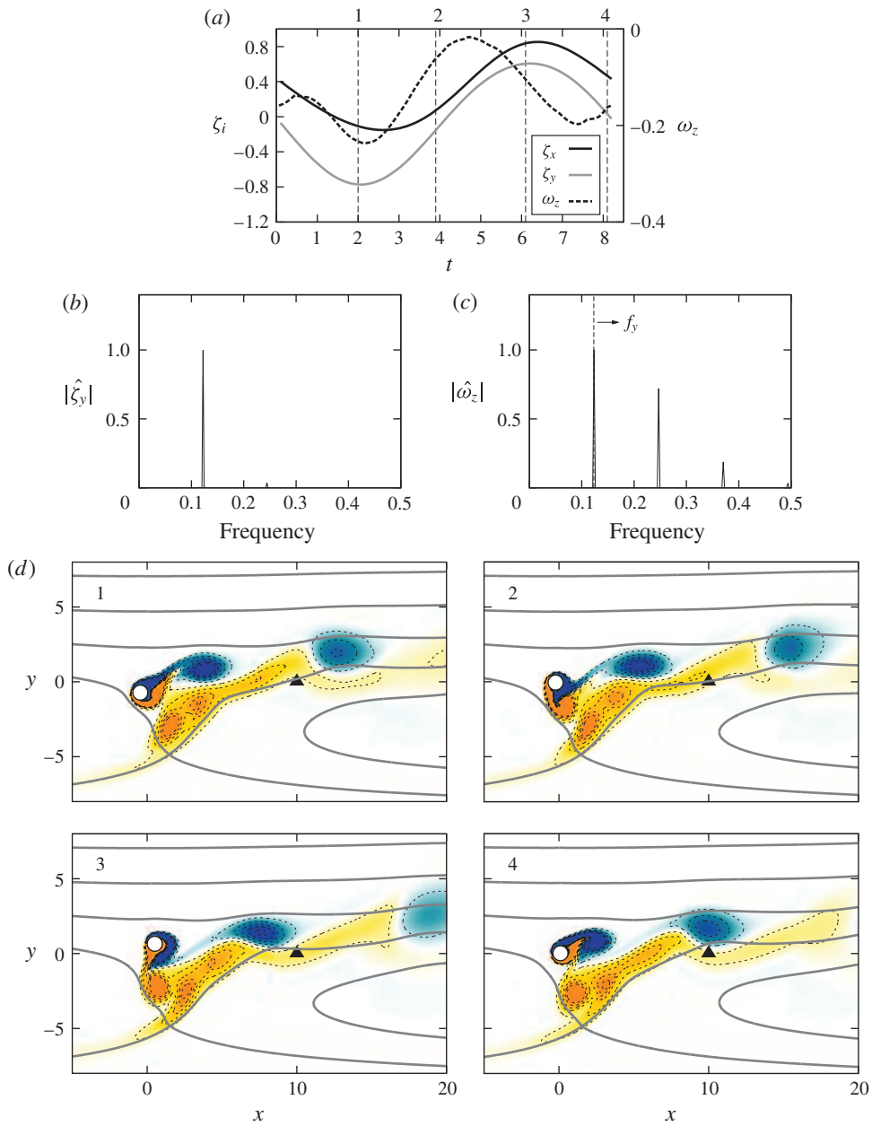
FIGURE 14. (Colour online) Same as figure 12 for regime VH1 , (\beta, U^*) = (0.3, 6) . In (d), the three positive vortices trapped in the saddle point region are labelled (snapshot 3).
