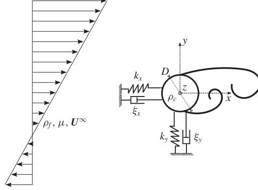
FIGURE 1. Sketch of the physical configuration.
