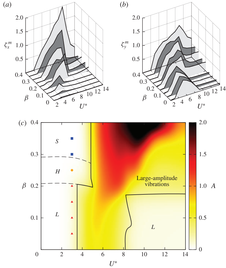
FIGURE 8. (Colour online) Body oscillation amplitudes: maximum (a) in-line and (b) cross-flow response amplitudes as functions of \beta and U^* , and (c) iso-contours of the typical oscillation amplitude A in the (\beta, U^*) parameter space. The region of large-amplitude responses ( A > 0.15 ) and regimes L , H and S in the absence of large-amplitude oscillations are indicated in (c). The coloured symbols in (c) indicate the selected points represented in figures 3(a) and 4(a).
