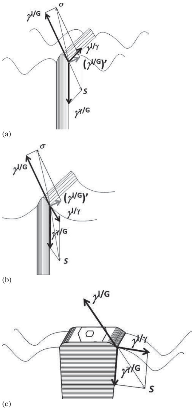
Fig. 8. Schematic of coupled growth of graphite when: (a) graphite grows along the prismatic direction with positive curvature of austenite at the triple junction; (b) graphite grows along the prismatic direction with negative curvature of austenite at the triple junction; and (c) graphite grows along the basal direction with positive curvature of austenite at the triple junction. The forces acting at the triple junction are shown in bold lines, their (near) equilibrium is illustrated with the thin lines.
