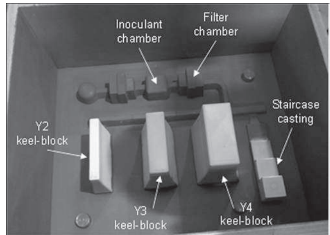
Fig. 2. Pattern used for preparing the poured castings.
