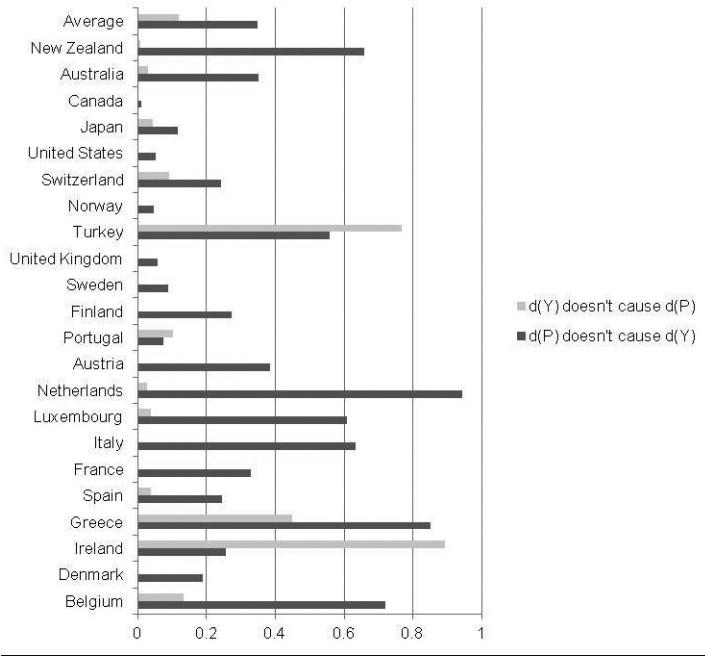
Figure 2. Probabilities of Granger non-causality (based on chi-sq stat.), allowing for linear trend, 1960–2015
