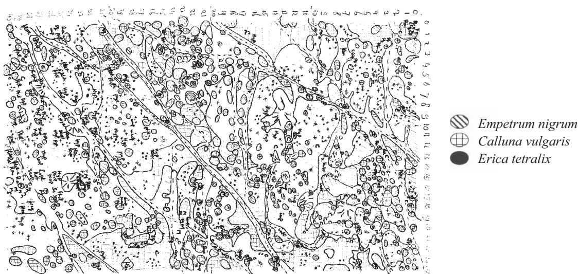
Figure 1. Vegetation map of the heathland in 1973 (10 years after fire). The dimensions are 12 m x 20 m. The most impressive changes in this period were the decrease in bare ground due to increasing plant cover and the increase of disturbance (emergence of sheep paths).
