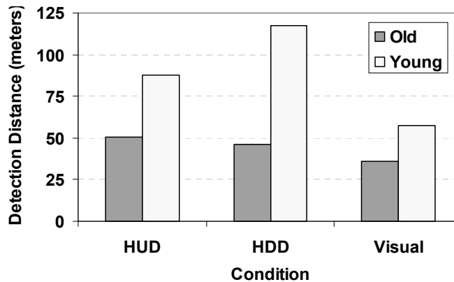
Figure 2. An interaction effect was observed between driver age and detection distance.
