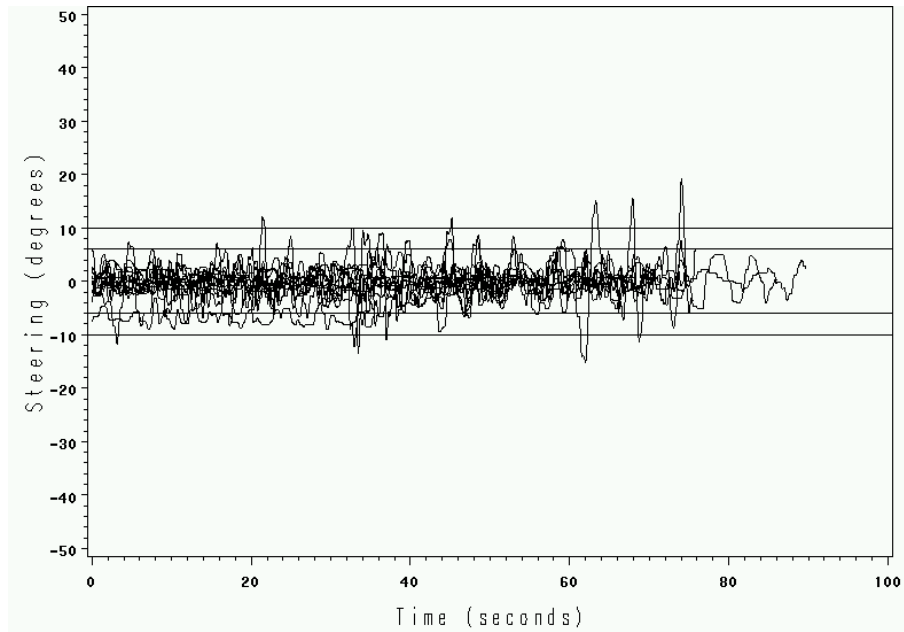
Figure 2. Time series of steering wheel position of all 13 drivers for the second segment.
