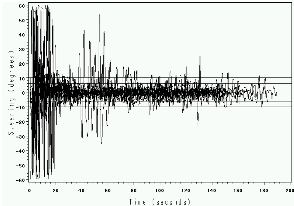
Figure 1. Time series of steering wheel position of all 13 drivers for the first segment.
