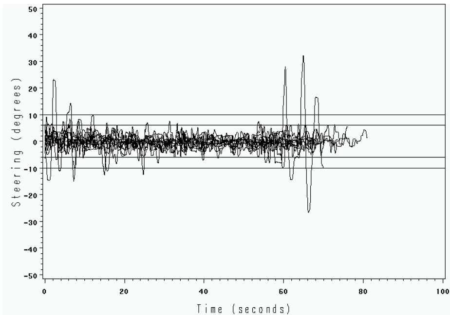
Figure 3. Time series of steering wheel position of all 13 drivers for the third segment.
