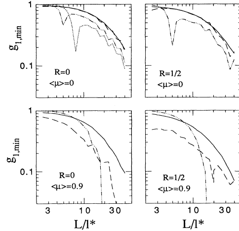
FIG. 8. Value of the correlation function above which the functional form of the predicted x dependence is accurate to 1%, i.e., g_{1Y}(x) evaluated where \chi(x) = 0.01 vs optical thickness L/l^* . The solid curves are for g_{1S}(x) of Eq. (6); the dashed curves are for g_{1DWS}(x) of Eq. (7); the dash-dotted curves are for g_{1(DWS)}(x) of Eq. (8); and the dotted curve is for g_{1CT}(x) of Eq. (9). Plots are labeled according to the boundary reflectivity R and the average cosine of the scattering angle \langle \mu \rangle .
