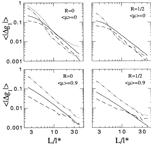
FIG. 5. Average absolute deviation between the approximate and benchmark correlation functions \langle |\Delta g_1| \rangle defined by Eq. (13) vs optical thickness L/l^* . The solid curves are for g_{1S}(x) of Eq. (6); the dashed curves are for g_{1DWS}(x) of Eq. (7); the dash-dotted curves are for g_{1(DWS)}(x) of Eq. (8); and the dotted curve is for g_{1CT}(x) of Eq. (9). Plots are labeled according to the boundary reflectivity R and the average cosine of the scattering angle \langle \mu \rangle .
