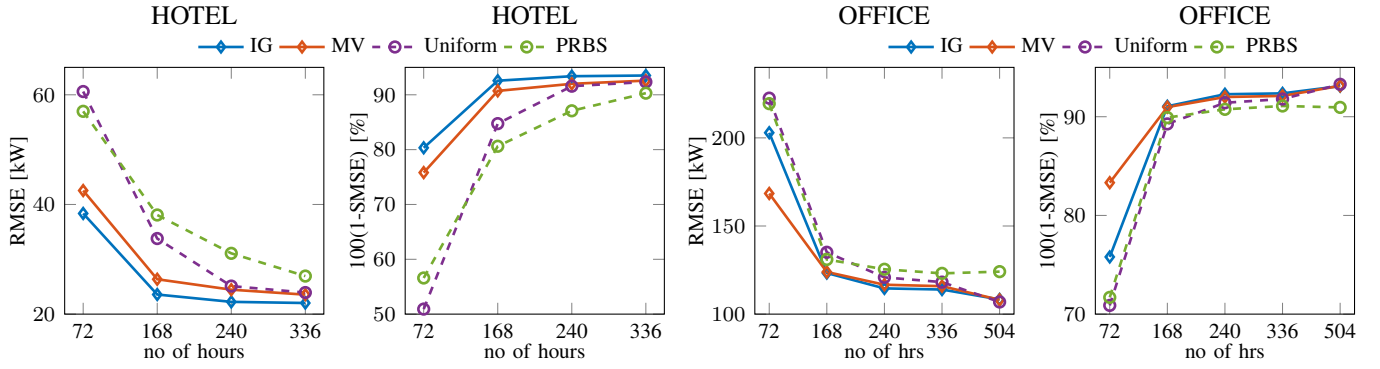
Fig. 5: Comparison of model accuracies for different experiments: OED based on information gain (IG), OED based on maximum variance (MV), uniform random sampling (Uniform) and pseudo random binary sampling (PRBS) for two buildings: hotel and office. RMSE denotes root mean square error and SMSE standardized mean square error; lower RMSE and higher 1-SMSE indicate better prediction accuracy.
