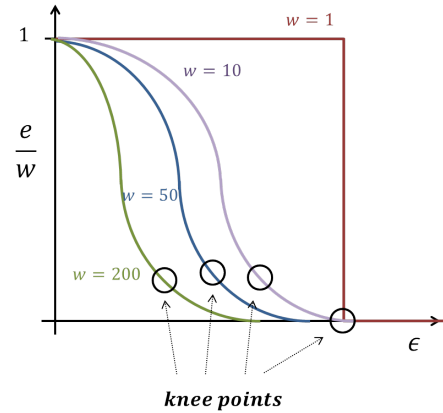
Figure 5: Sample plots of the proportion of faults in a window ( e/w ) against the error bound ( \epsilon ).
