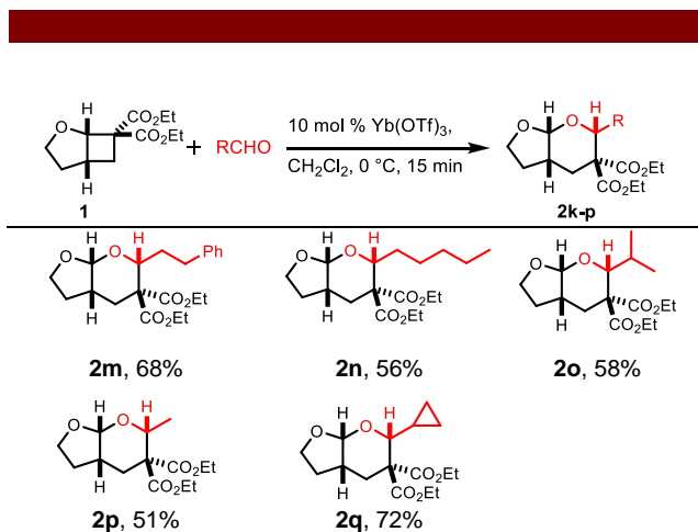
Figure 2. [4+2] Cycloaddition of DA cyclobutanes and Aliphatic Aldehydes
