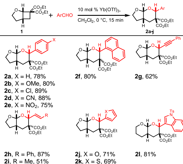
Figure 1. [4+2] Cycloaddition of DA cyclobutanes and Aromatic and Heteroaromatic Aldehydes
