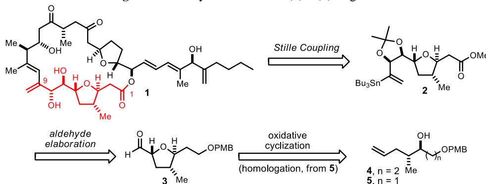
Figure 1. Retrosynthesis of the C(1)-C(9) fragment
