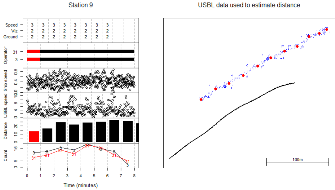
Figure 2: FU15 western Irish Sea grounds: R - tool quality control plot for station 9 of the 2017 survey.
