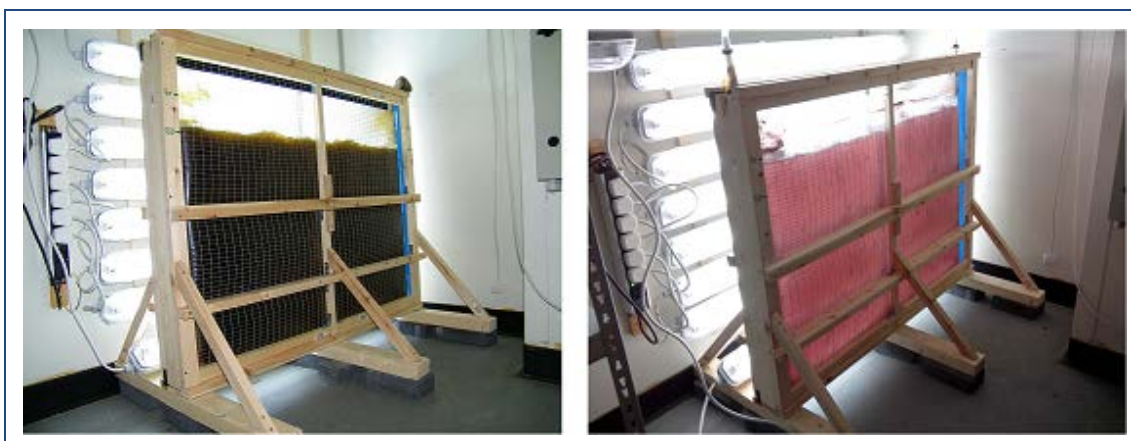
Figure 16 Low cost flat-panel photobioreactors (FP-PBRs) developed to assess large-scale production of microalgae under controlled conditions. Batch-cultures of the diatom P. tricornutum (left) and the red microalga P. purpureum (right)
