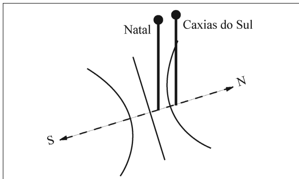
Fig. 3. Fixing the shadows and moving the gnomons. This diagram is similar to that of Fig. 1, but now for gnomons placed on different latitudes. The one on the equator (Lat: 0°) would be placed on the straight middle line, as required by symmetry. Those located to the south of the equator, for example in Natal (Lat: 5.8°S) and in Caxias do Sul (Lat: 29.2°S), are shown in the diagram. One gnomon located in Buenos Aires (Lat: 34.5°S) would be placed further to the right of these. Hence, shadows observed in Caxias do Sul or in Buenos Aires at noon can never point toward the north. (Although we know that the declination lines are slightly modified if we change the latitude of observers located not very far from the equator; here, for simplicity, we considered them unchanged.)
