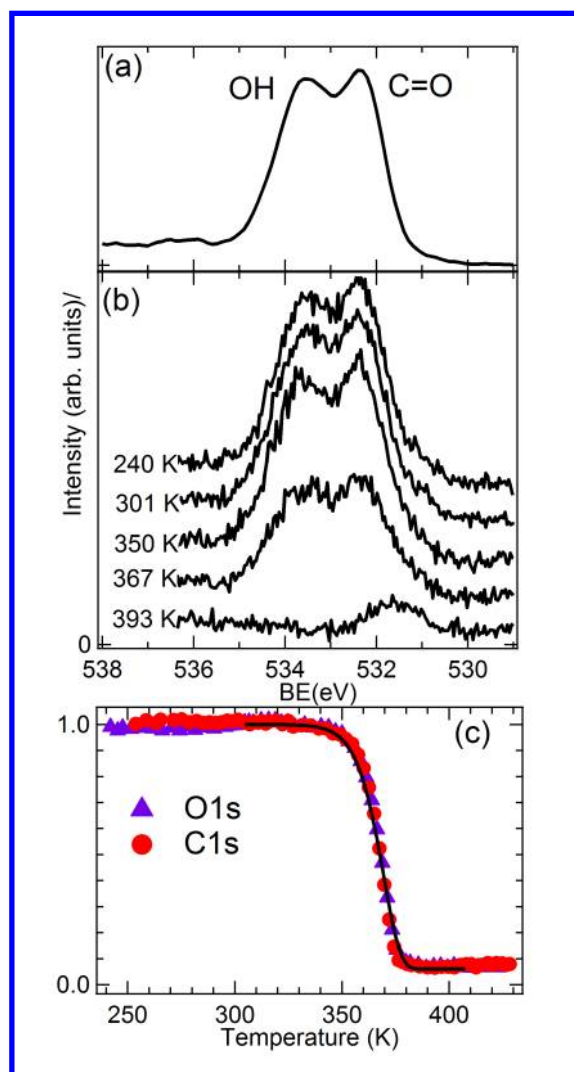
Figure 2: a) O1s photoemission spectra obtained for a submonolayer coverage of TPA on the 0.5 ML Sn/Cu surface alloy at room temperature b) series of O1s spectra measured as a function of the substrate temperature using a fast-XPS mode. c) Total intensity of the O1s and C1s spectra vs substrate temperature. The continuous black line corresponds to a first-order Polanyi-Wigner model (see text and the SI).
