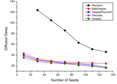
(b) Ego-Facebook
