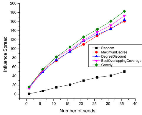
(a) NetHEPT
