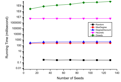
(b) Ego-Facebook
