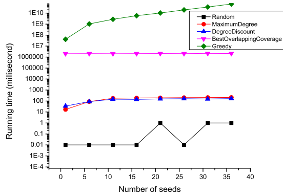
(c) Wiki-vote
