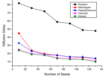
(c) Wiki-vote
