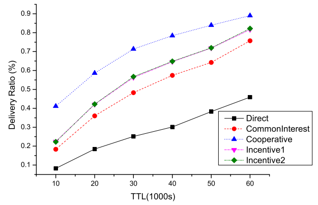
(b) INFOCOM06
