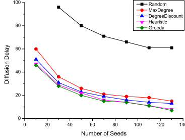
(a) NetHEPT
