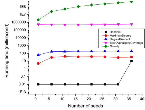
(b) Ego-Facebook
