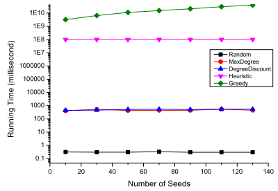
(c) Wiki-vote
