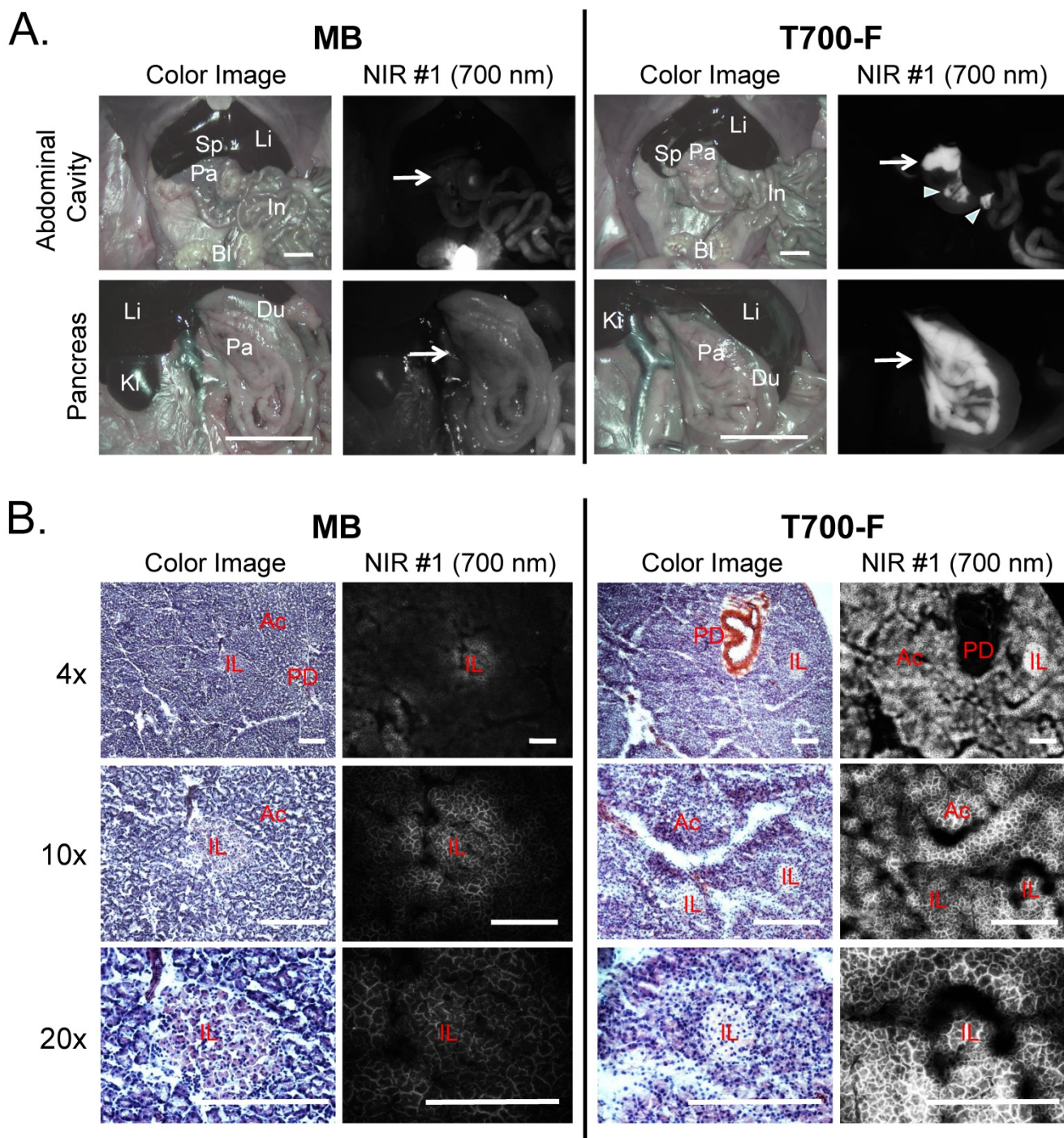
Figure 3. Intraoperative Pancreas Imaging in SD Rats: a) 1.2 \mu mol of MB and 100 nmol of T700-F were injected intravenously 15 min and 4 h prior to imaging, respectively (n = 3). Abbreviations used are: Bl, bladder; Du, duodenum; In, intestine; Ki, kidney; Li, liver; Pa, pancreas; Sp, spleen. Arrows indicate pancreas and arrowheads indicate autofluorescence of food in lumen of intestine. Scale bars = 1 cm. All NIR fluorescence images have identical exposure times and normalizations. b) Histological analysis: Consecutive sections from rat pancreas stained with H&E or unstained were observed using an NIR fluorescence microscope. Abbreviations used are: Ac, acinus; IL, islets of Langerhans; PD, pancreatic duct. Scale bars = 300 \mu m. All NIR fluorescence images for each condition have identical exposure times and normalizations.
