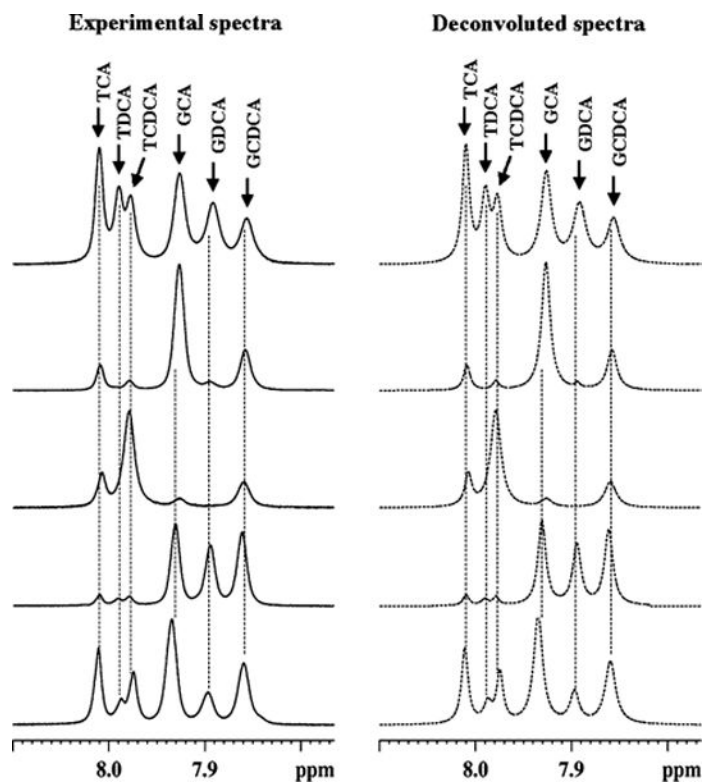
Fig. 2. Left Portions of the 800 MHz ^1\text{H} -NMR spectra of gallbladder bile from five different patients (four from non-liver disease controls and one from hepatitis C patient). The spectra were obtained by decoupling methylene protons of glycine-/taurine-conjugated bile acids. Right The corresponding deconvoluted spectra obtained for estimating the integrals. GCA glycocholic acid; GCDCA glycochenodeoxycholic acid; GDCA glycodeoxycholic acid; TCA taurocholic acid; TCDCA : taurochenocholic acid and TDCA taurodeoxycholic acid
