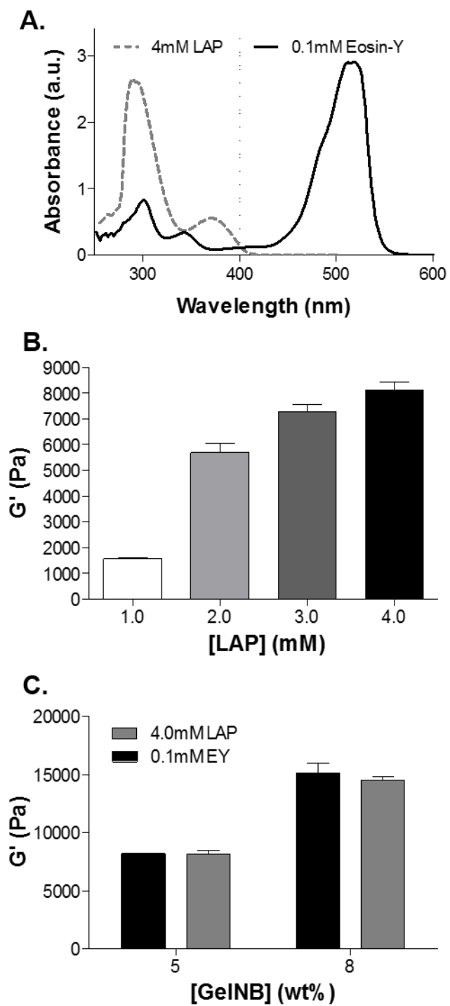
Figure 2. (A) UV/vis spectra of LAP/eosin-Y. (B) Shear moduli of 5 wt% GeINB hydrogel crosslinked by 2.8 wt% PEG4SH using different concentrations of LAP. (C) Shear moduli of 5 wt% and 8 wt% (R=1.0) GeINB hydrogels initiated by LAP or EY.
