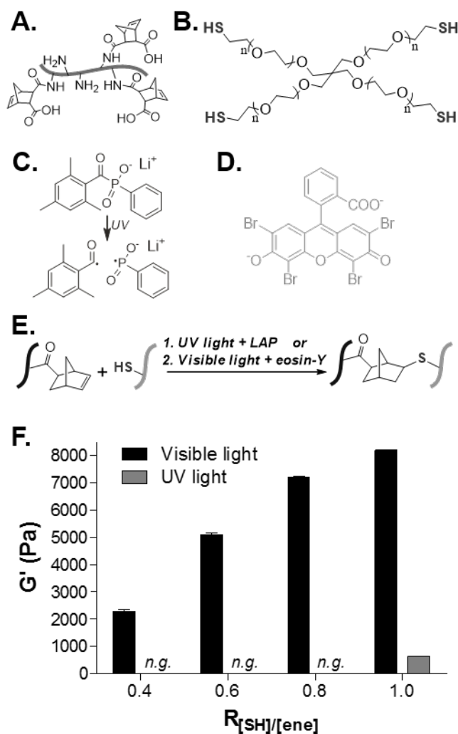
Figure 1. Chemical structures of: (A) norbornene-functionalized gelatin (GelNB), (B) PEG-tetra-thiol (PEG4SH), (C) cleavage type photoinitiator lithium acylphosphinate (LAP), and (D) non-cleavage type photoinitiator eosin-Y (EY). (E) Schematic of thiol-norbornene photoclick reaction using two initiation systems: 1. UV light + LAP and 2. Visible light + eosin-Y. (F) Shear moduli of 5 wt% GelNB (i.e. 11.1 mM norbornene) hydrogels crosslinked by PEG4SH at different thiol-to-ene molar ratios ( R_{[SH]}/[ene] ). Gelation was initiated via either visible light + 0.1 mM EY or UV light + 0.1 mM LAP ( n.g. : no gel).
