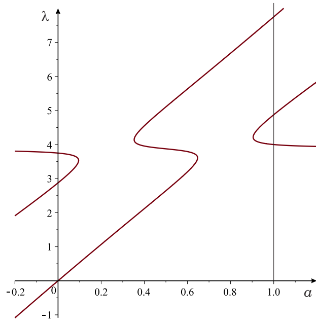
Figure 24: \alpha_1 = \alpha_2 = 3 , \alpha_0 = \alpha_3 = 15/8
