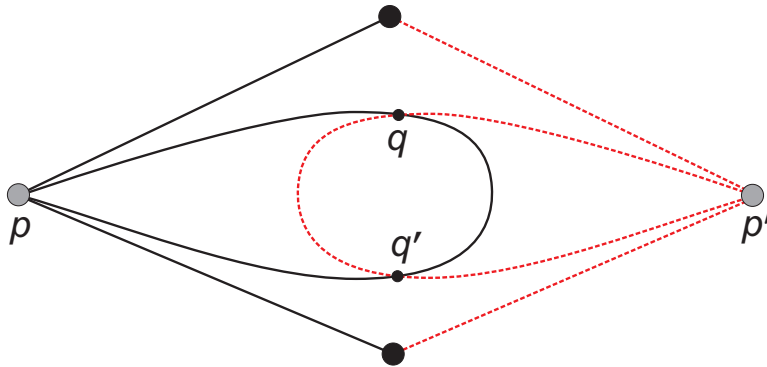
Figure 2: Pseudo-diagonal connecting two integer corners of Q .
