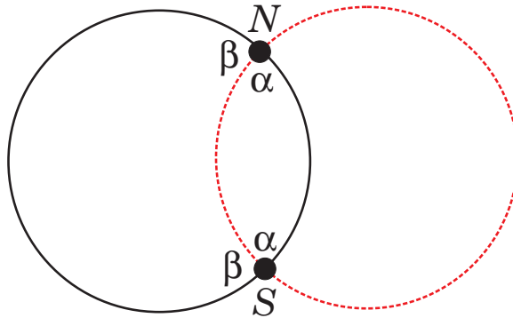
Figure 1: Partition \mathcal{P} of the Riemann sphere by two circles.
