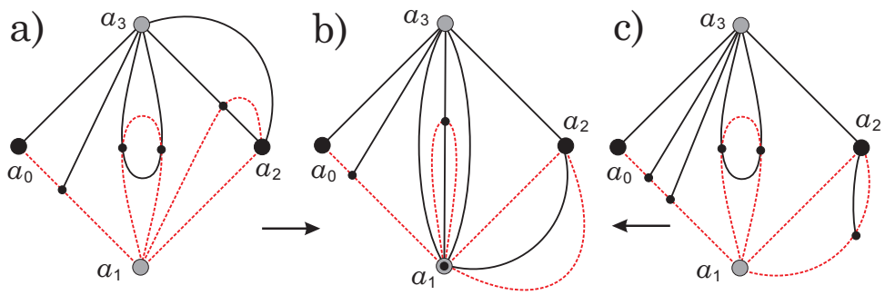
Figure 19: An aa-chain of quadrilaterals of length 1.
