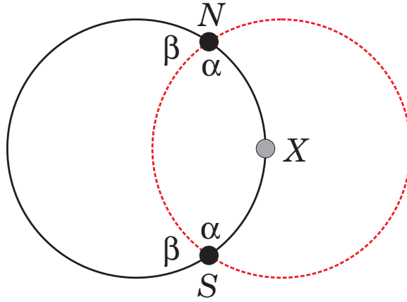
Figure 3: Location of the point X .
