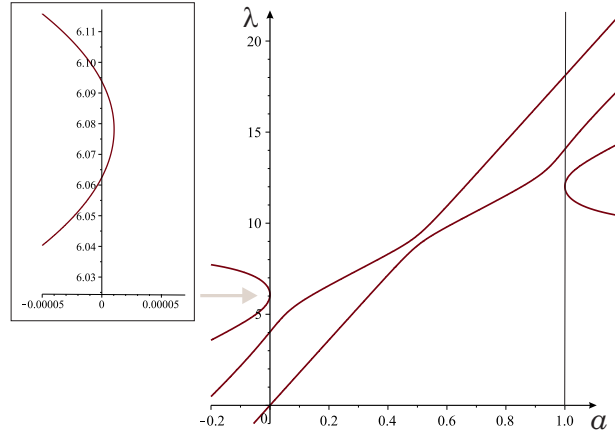
Figure 20: \alpha_1 = 4 , \alpha_2 = 6 , \alpha_0 = \alpha_3 = 65/32
