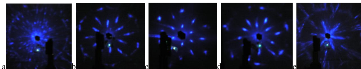
Figure 7. Characteristic blue laser ( \lambda=325\text{nm} ) diffraction patterns recorded in reflection from monolayers of 390nm spheres self-assembled at different pH factor of water. From left to right: pH = 2.8, 3.7, 4.1, 4.9 and 5.5. The size of the laser spot is approximately 3mm.
