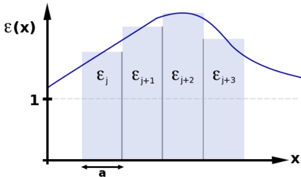
FIG. 1: The medium is assumed inhomogeneous along x and is divided into N homogeneous slices of width a . The local value of the regularised stress tensor, (1) is then investigated within the medium in the limit as a \rightarrow 0 . For the purposes of illustration only the permittivity, \epsilon , is shown here. Our analysis holds for both inhomogeneous permittivity and permeability.
