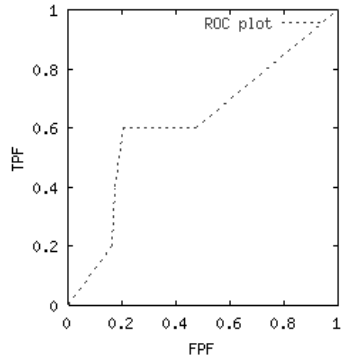
ROC curve for fold_2
