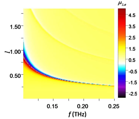
FIG. 4. (Color online) The effective permeability \mu_{\perp e} is plotted as a function of the frequency and dimensionless thickness l , for the same assumptions and parameter values as in Fig. 3.
