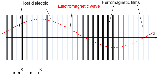
FIG. 1. (Color online) The sketch of the proposed metamaterial is schematically shown. Thin ferromagnetic layers are separated by layers of the host dielectric. The electromagnetic wave (light) propagates along z direction. The light wavelength is much greater than the characteristic dimensions of the superlattice.
