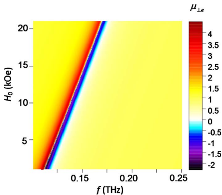
FIG. 7. (Color online) The effective permeability \mu_{\perp e} is plotted as a function of the frequency and bias magnetic field H_0 , for the same assumptions and parameter values as in Fig. 3 (spins are perfectly pinned at one side of the film).
