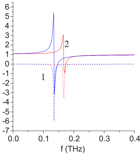
FIG. 3. (Color online) The calculated effective permeability is shown as a function of frequency for the cases of (1) in-plane and (2) out-of-plane magnetizations. The solid and dashed lines denote the real and imaginary parts of the effective permeability, respectively. The effective permeability is calculated for an array of CoFe films with thickness of 5 nm. The filling fraction of 0.25 is assumed. The spins are perfectly pinned at one surface of the film and are free at the other.
