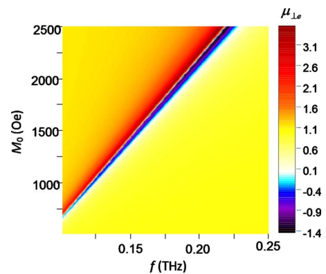
FIG. 5. (Color online) Effective permeability \mu_{\perp e} is plotted as a function of the frequency and magnetization of saturation M_0 , for the same assumptions and parameter values as in Fig. 3.
