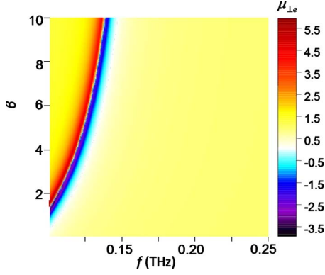
FIG. 6. (Color online) The effective permeability \mu_{\perp e} is plotted as a function of frequency and pinning parameter \beta . The calculations are for the same assumptions and parameter values as in Fig. 3, except the finite pinning strength assumed here.
