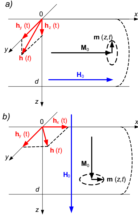
FIG. 2. (Color online) The magnetic geometry of the ferromagnetic layers is shown for the (a) in-plane and (b) out-of-plane magnetizations.
