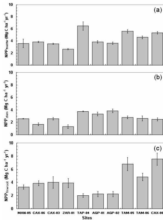
Fig. 3. The net primary productivity of the major subcomponents of the NPP_{total} in the ten studied sites: (a) fine litter production; (b) stem production; and (c) fine root production. All values are in Mg\ C\ ha^{-1}\ yr^{-1} with their respective standard errors. Sites are ranked by increasing soil available phosphorus (Table 2).
