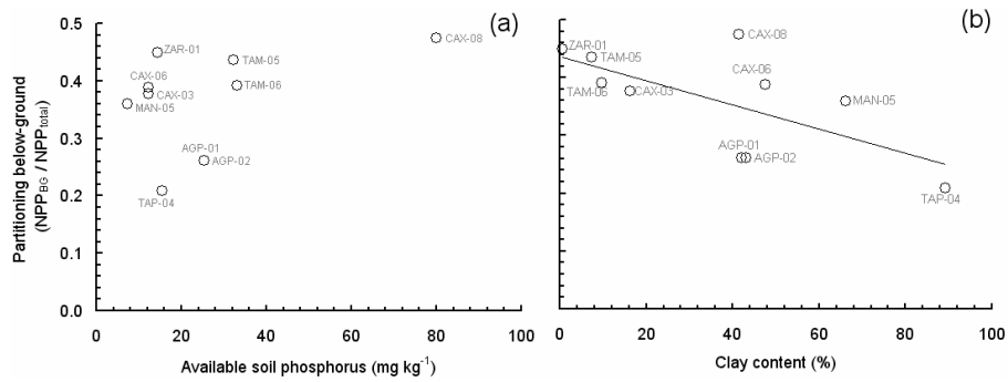
Fig. 8. The relationship between the proportion of NPP total allocated below-ground (NPP BG /NPP total ) and (a) available soil phosphorus concentration and (b) soil clay content. The regression line in black indicates a significant relationship ((NPP BG /NPP total ) = -0.0021(\pm 0.008) \times \text{Clay} + 0.44(\pm 0.04) , R^2 = 0.44 , N = 10 , P = 0.04 ).
