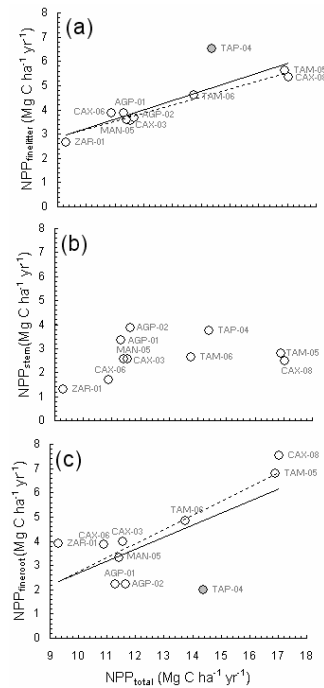
Fig. 5. The relationship between (a) NPP_{finelitter} and the total NPP, with the regression lines for all data (black) and without the Tapajós site (black dashed) (all data – NPP_{finelitter}=0.38(\pm 0.08) \times NPP_{total}-0.60(\pm 1.07) , N=10 , R^2=0.73 , P=0.001 ; without Tapajós – NPP_{finelitter}=0.34(\pm 0.03) \times NPP_{total}-0.18(\pm 0.39) , N=9 , R^2=0.95 , P<0.001 ); (b) NPP_{stem} and the total NPP (no significant); (c) NPP_{fineroot} and total NPP, with the regression lines for all data (black) and without the Tapajós site (black dashed) (all data – NPP_{fineroot}=0.49(\pm 0.18) \times NPP_{total}-2.26(\pm 2.42) , N=10 , R^2=0.47 , P=0.03 ; without Tapajós – NPP_{fineroot}=0.58(\pm 0.13) \times NPP_{total}-3.02(\pm 1.73) , N=9 , R^2=0.73 , P=0.003 ).
