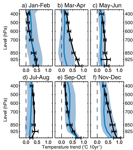
Figure 2. Vertical profile of Arctic-mean temperature trends (1979–2008) for (a) Jan–Feb, (b) Mar–Apr, (c) May–Jun, (d) Jul–Aug, (e) Sep–Oct, and (f) Nov–Dec. The black lines denote the reanalysis ensemble-mean trends and the whiskers show the reanalysis ensemble spread. The blue lines denote the model ensemble-mean trends from the GLB experiment and the shaded envelopes show the model ensemble spread.
