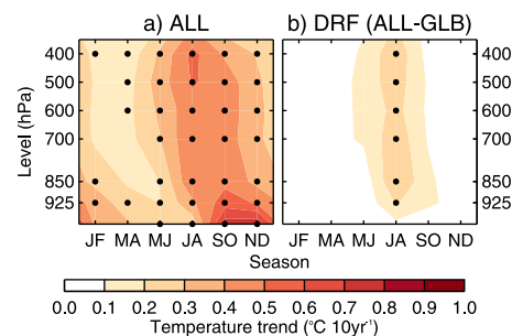
Figure 4. (a) Vertical and seasonal structure of the ensemble-mean Arctic-mean temperature trends (1979–2008) in the ALL experiment. (b) As in Figure 4a, but for difference between the ALL and GLB experiments. Black dots show trends that are statistically significant at the 95% level ( p < 0.05 ).
