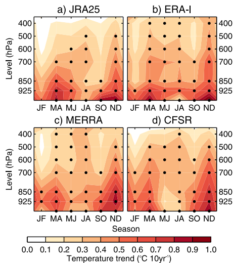
Figure 1. Vertical and seasonal structure of Arctic-mean temperature trends (1979–2008) in the (a) JRA25, (b) ERA-I, (c) MERRA and (d) CFSR reanalyses, respectively. Black dots show trends that are statistically significant at the 95% level ( p < 0.05 ) based on a two-tailed student's t -test.
