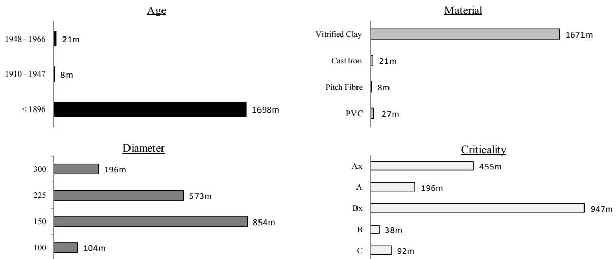
Figure 3: Sewer characteristics
