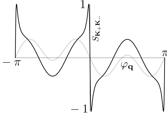
Figure 2.9: For the fixed frequency of excitation, \nu = 0.6 |t|/h , the degree of valley polarisation for two different polarisation angles \varphi_e = 0 (black line) and \varphi_e = \pi/2 (grey line) is shown. (Note, though it is possible to achieve full valley polarisation i.e. S_{\mathbf{K}\mathbf{K}'} = 1 , at such values of \varphi_{\mathbf{q}} the angular generation density is limited.)
