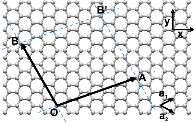
Figure 3.1: An unrolled carbon nanotube. The cylinder is formed by rolling the graphene sheet such that points O and A and points B and B' coincide with one another. The vectors OA and OB' define the vectors \mathbf{C}_h and \mathbf{T} respectively. \mathbf{a}_1 and \mathbf{a}_2 are the graphene primitive lattice vectors.
