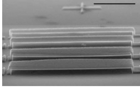
Figure 4.4: A series of top gates of varying sizes separated from the substrate with an air gap. The scale bar is 2\mu\text{m} . From Liu et al. in Ref. [22]
