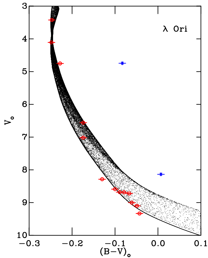
Figure 2.10: The best-fitting V_0, (B - V)_0 CMD for \lambda Ori, with an age of 10.0 Myr and distance modulus dm = 8.02 . The probability density \rho is shown as the greyscale isochrone. Circles represent the photometric data of Murdin & Penston (1977). The plotted uncertainties are the magnitude independent values discussed in Section 2.8.3. Asterisks represent stars that were clipped before deriving the best-fit (see text).
