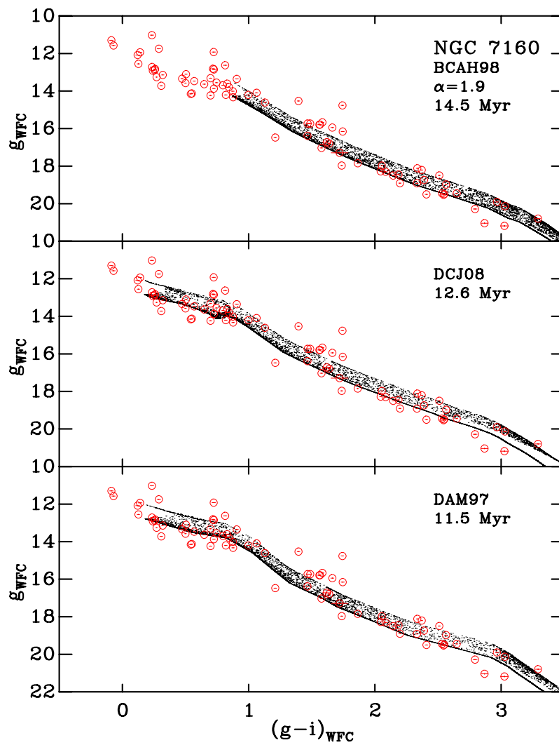
Figure 5.10: Pre-MS stars selected as members of NGC 7160. Circles are Li I and H \alpha spectroscopic, IR excess, and extinction-based members from Sicilia-Aguilar et al. (2006a). Overlaid are the best-fitting isochrones of BCAH98 \alpha = 1.9 (upper panel), DCJ08 (middle panel), and DAM97 (lower panel) at the best-fit MS distance. The probability densities \rho are shown as the greyscale isochrones.
