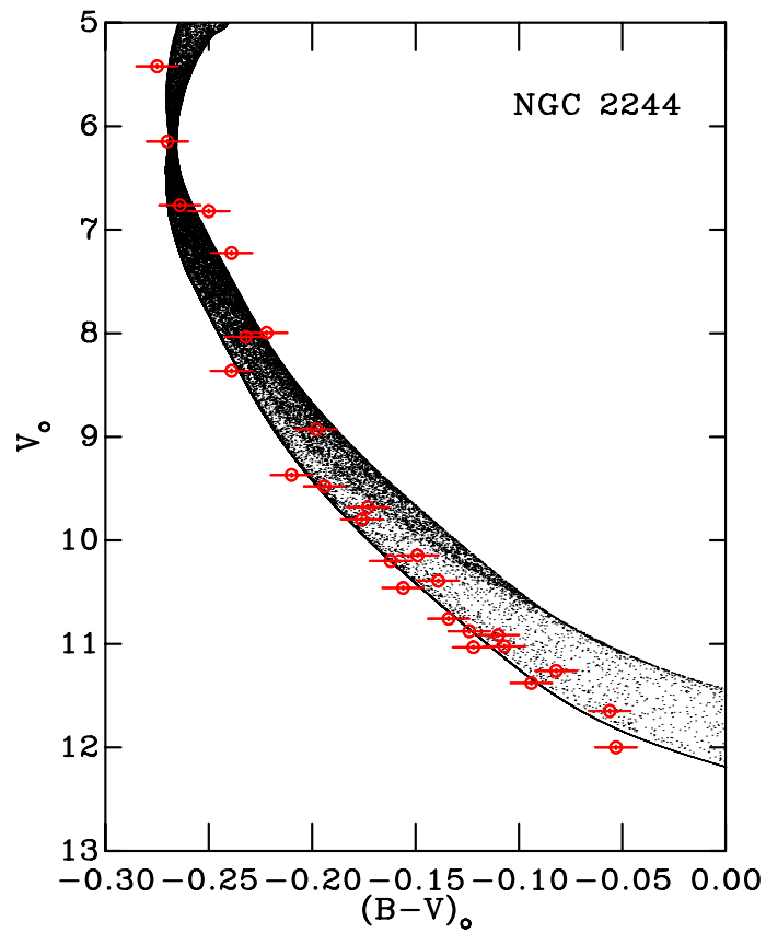
Figure 2.21: The best-fitting V_0, (B - V)_0 CMD for NGC 2244, with an age of 6.6 Myr and distance modulus dm = 10.70 . The probability density \rho is shown as the greyscale isochrone. Circles represent the photometric data of Johnson (1962). The plotted uncertainties are the magnitude independent values discussed in Section 2.8.4.6.
