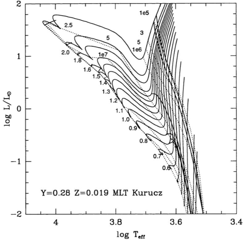
Figure 1.6: Schematic of evolutionary mass tracks on the H-R diagram for low-mass pre-MS stars. Solid lines are evolutionary tracks for masses 0.3\text{--}2.5 M_{\odot} . Dotted lines represent isochrones ranging in age from 10^5 - 10^7 years. The upper continual line illustrates the average sequence of deuterium burning. The point at which the evolutionary tracks cease (note the numerals on the left-hand side of each track) denotes the point at which said star has reached the ZAMS. These models are based on solar abundances. Reproduced with permission from the AAS. Credit: D’Antona & Mazzitelli (1994).
