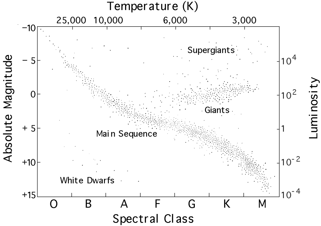
Figure 1.5: A Hertzsprung-Russell diagram illustrating the three main population regions; i) main-sequence (dwarf) stars, ii) the giant stars and iii) the white dwarf stars. Credit: Phil Newman, http://heasarc.gsfc.nasa.gov/docs/RXTE_Live/class.html .
