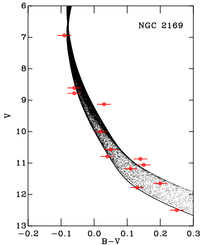
Figure 2.19: The best-fitting V, B - V CMD for NGC 2169 using the updated Geneva-Bessell isochrones, with an age of 12.6 Myr and distance modulus dm = 9.99 . The probability density \rho is shown as the greyscale isochrone. Circles represent the photometric data of Hoag et al. (1961). The plotted uncertainties are the magnitude independent values discussed in Section 2.8.4.5.
