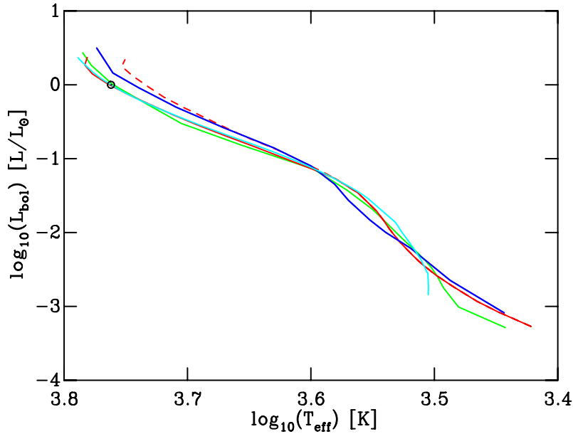
Figure 4.2: Variations in the pre-MS isochrones at an age of 4.6 Gyr for the models adopted in this work; BCAH98 \alpha = 1.9 (red, continuous), BCAH98 \alpha = 1.0 (red, dashed), SDF00 (blue), DCJ08 (cyan) and DAM97 (green). The small solar symbol denotes the solar values of L_{\text{bol}} and T_{\text{eff}} .
