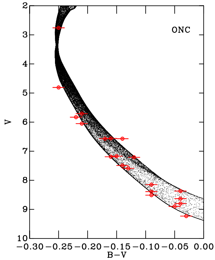
Figure 2.31: The best-fitting V, B - V CMD for stars in the vicinity of the ONC, with an age of 6.0 Myr and distance modulus dm = 7.94 . The probability density \rho is shown as the greyscale isochrone. Circles represent the photometric data of Walker (1969), with the associated uncertainties shown as the bars.
