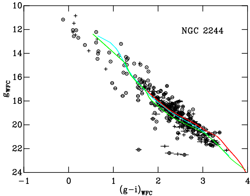
Figure 5.12: NGC 2244 g_{\text{WFC}}, (g-i)_{\text{WFC}} CMD with stars selected as pre-MS members. Circles are the X-ray sources from Wang et al. (2008) and crosses are IR excess objects from Balog et al. (2007). Semi-empirical BCAH98 \alpha = 1.9 (red), DCJ08 (cyan) and DAM97 (green) isochrones at ages of 2 Myr are overlaid at a distance modulus dm = 10.70 and reddened by E(B-V) = 0.43 according to the prescription described in Section 5.5. Note how all three isochrones do not follow the shape of the observed pre-MS locus.
