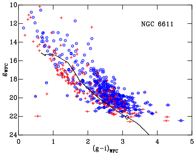
Figure 5.18: Same as Fig. 5.13 but for NGC 6611. Circles are the X-ray sources from Guarcello et al. (2007) and the crosses are IR excess sources from Guarcello et al. (2009). The 6 Myr model isochrone is at a distance modulus dm = 11.38 and reddened by E(B - V) = 0.71 .
