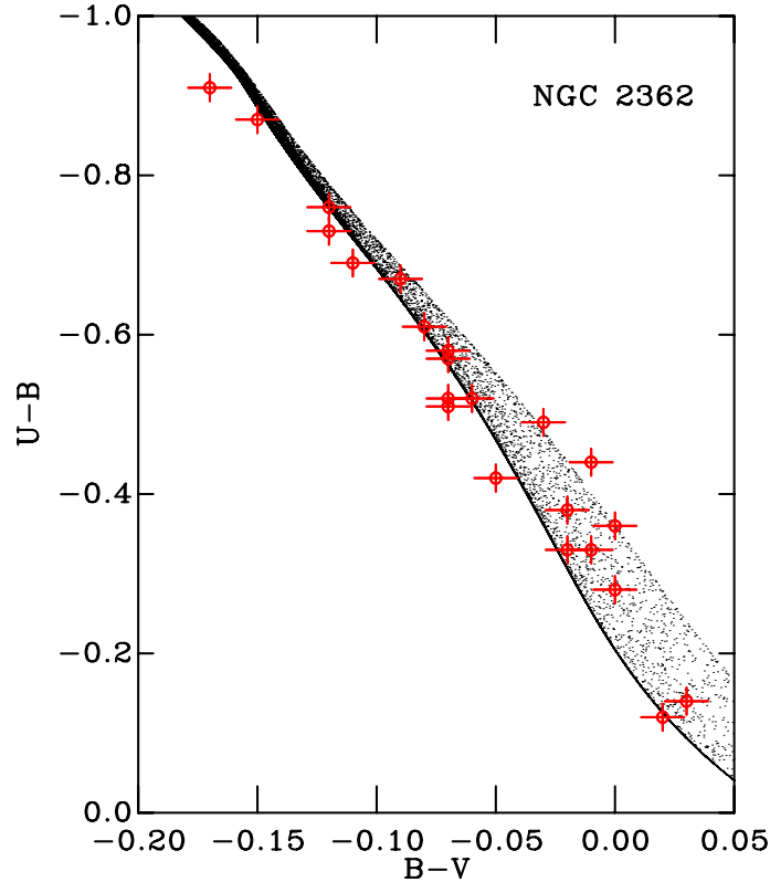
Figure 2.22: The best-fitting U - B, B - V colour-colour diagram for NGC 2362, with a reddening E(B - V) = 0.07 . The probability density \rho is shown as the greyscale isochrone. Circles represent the photometric data of Johnson & Morgan (1953), with the associated uncertainties shown as the bars.
