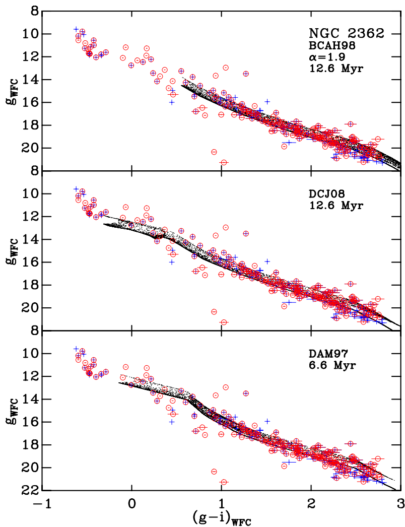
Figure 5.8: Pre-MS stars selected as members of NGC 2362. Crosses are the combined Li I and H \alpha spectroscopic and IR excess sources from Dahm & Hillenbrand (2007) and circles are X-ray sources from Damiani et al. (2006a). Overlaid are the best-fitting isochrones of BCAH98 \alpha = 1.9 (upper panel), DCJ08 (middle panel), and DAM97 (lower panel) at the best-fit MS distance. The probability densities \rho are shown as the greyscale isochrones.
