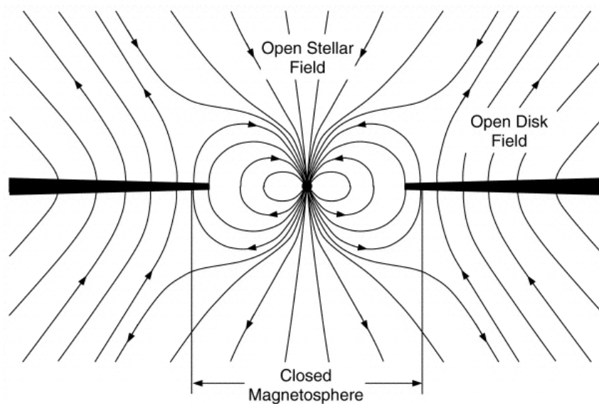
Figure 1.3: An idealised representation of the magnetic field structure of a CTTS. There are three discrete regions of field; i) closed field lines close to the stellar surface that contain the coronal plasma, ii) closed field lines that thread the circumstellar disc and permit accretion flows onto the stellar surface and iii) open field lines which support outflows. Reproduced with permission from the AAS. Credit: Goodson et al. (1997).
