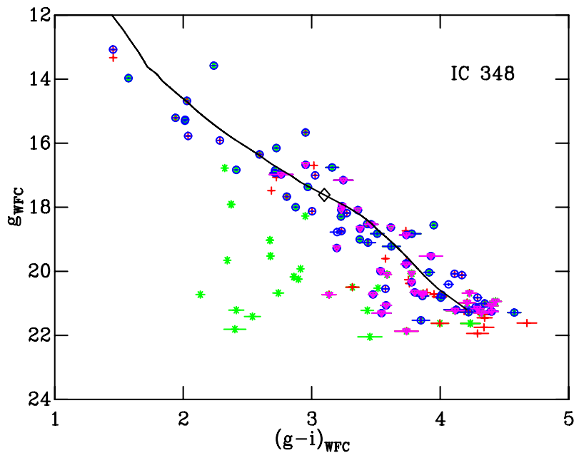
Figure 5.14: Same as Fig. 5.13 but for IC 348. Circles are the X-ray sources from Preibisch & Zinnecker (2002), the crosses are the \text{H}\alpha , Na I, and K I spectroscopic members from Luhman et al. (2003, 2005a,b), the triangles are the \text{H}\alpha spectroscopic members from Herbig (1998), and the asterisks are the combined periodic variable sources from Cohen et al. (2004) and Littlefair et al. (2005). The 6 Myr model isochrone is at a distance modulus dm = 6.98 and reddened by E(B-V) = 0.69 .
