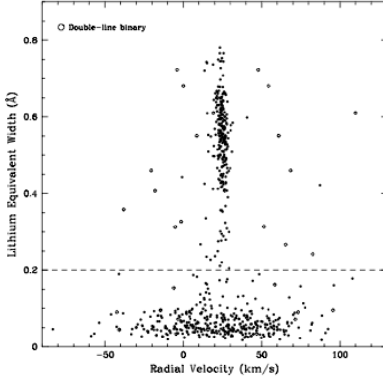
Figure 1.8: Equivalent width of Li I against radial velocity for stars around the \lambda Ori SFR. Those with W_{\lambda}(\text{Li I}) > 0.2 \text{ \AA} and clustered about the mean radial velocity are taken to be pre-MS members. Reproduced with permission from the AAS. Credit: Dolan & Mathieu (2001).
