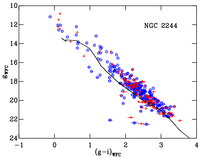
Figure 5.16: Same as Fig. 5.13 but for NGC 2244. Circles are the X-ray sources from Wang et al. (2008) and the crosses are IR excess objects from Balog et al. (2007). The 6 Myr model isochrone is at a distance modulus dm = 10.70 and reddened by E(B - V) = 0.43 .
