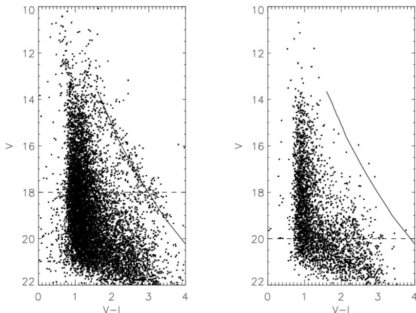
Figure 1.7: Left: The V, (V - I_c) CMD of the central 0.89 \text{ deg}^2 of the \sigma Ori cluster. The solid line is a 2.5 Myr isochrone (Baraffe et al. 1998, 2001) at a distance of 440 pc (Brown et al. 1994). The isochrone denotes the expected location of the pre-MS population of the Orion OB1b association. Right: The same CMD but for a control field with a smaller ( 0.29 \text{ deg}^2 ) FOV. The isochrone is the same as in the left panel. The dashed line in both cases represents the completeness limit of the data. Reproduced with permission from the AAS. Credit: Sherry et al. (2004).
