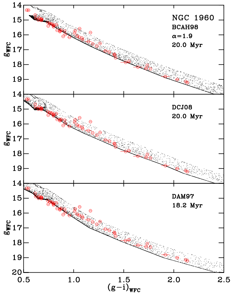
Figure 5.11: Pre-MS stars selected as members of NGC 1960. Circles are Li I spectroscopic members from Jeffries et al. (in preparation). Overlaid are the best-fitting isochrones of BCAH98 \alpha = 1.9 (upper panel), DCJ08 (middle panel), and DAM97 (lower panel) at the best-fit MS distance. The probability densities \rho are shown as the greyscale isochrones.
