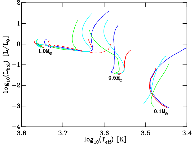
Figure 4.1: Variations in the pre-MS evolutionary tracks for masses of 0.1, 0.5 and 1.0 M_{\odot} for the models adopted in this work; BCAH98 \alpha = 1.9 (red, continuous), BCAH98 \alpha = 1.0 (red, dashed), SDF00 (blue), DCJ08 (cyan) and DAM97 (green). The small solar symbol denotes the solar values of L_{\text{bol}} and T_{\text{eff}} . Note that for masses < 0.6 M_{\odot} both computations of the BCAH98 models are identical, this is due to the insensitivity to the adopted mixing length parameter \alpha in this mass regime.
