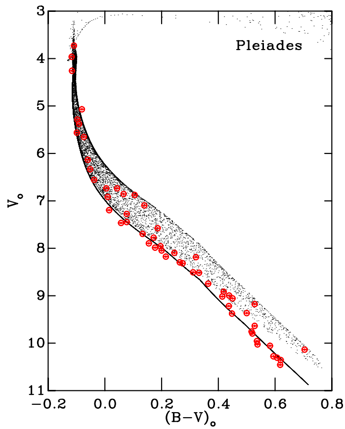
Figure 2.35: The best-fitting V_o , (B-V)_o CMD for the Pleiades, with an age of 131.8 Myr and distance modulus dm = 5.63 . The probability density \rho is shown as the greyscale isochrone. Circles represent the photometric data of Johnson & Morgan (1953), with the associated uncertainties shown as the bars.
