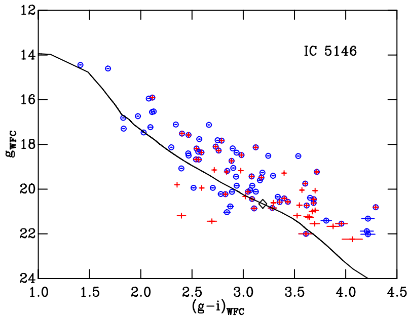
Figure 5.15: Same as Fig. 5.13 but for IC 5146. Circles are the IR excess sources of Harvey et al. (2008) and the crosses are spectroscopic members from Herbig & Dahm (2002). The 6 Myr model isochrone is at a distance modulus dm = 9.81 and reddened by E(B - V) = 0.75 .
