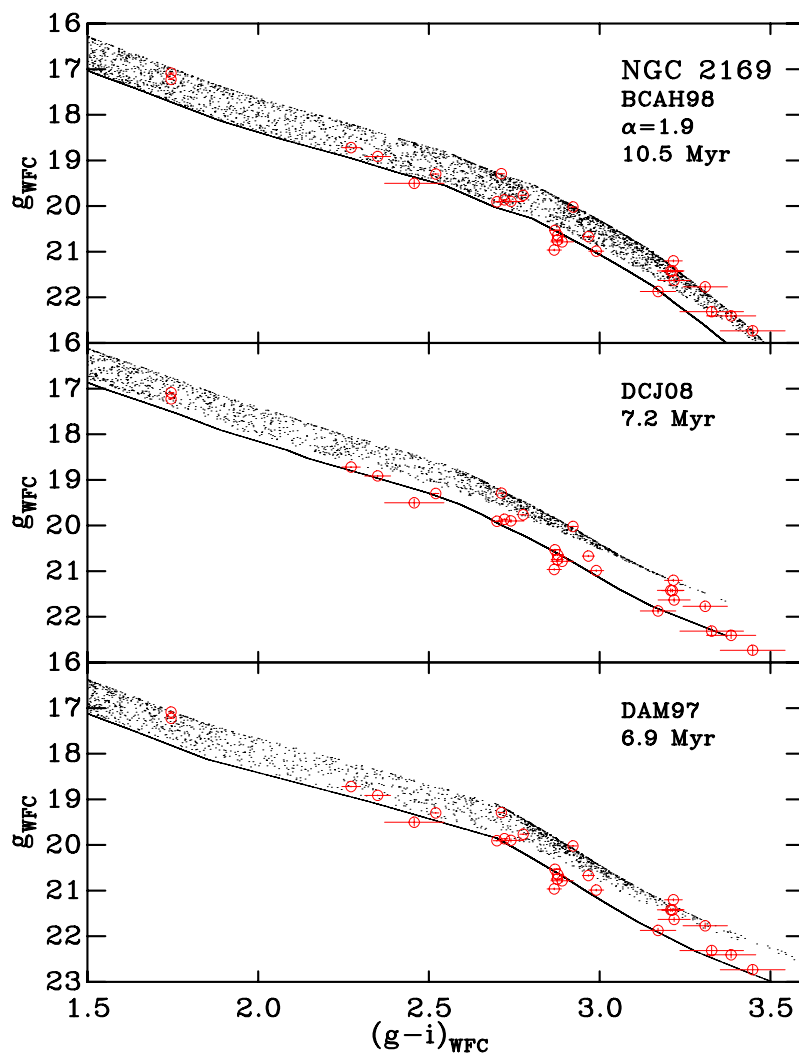
Figure 5.9: Pre-MS stars selected as members of NGC 2169. Circles are Li I spectroscopic members from Jeffries et al. (2007). Overlaid are the best-fitting isochrones of BCAH98 \alpha = 1.9 (upper panel), DCJ08 (middle panel), and DAM97 (lower panel) at the best-fit MS distance. The probability densities \rho are shown as the greyscale isochrones.
