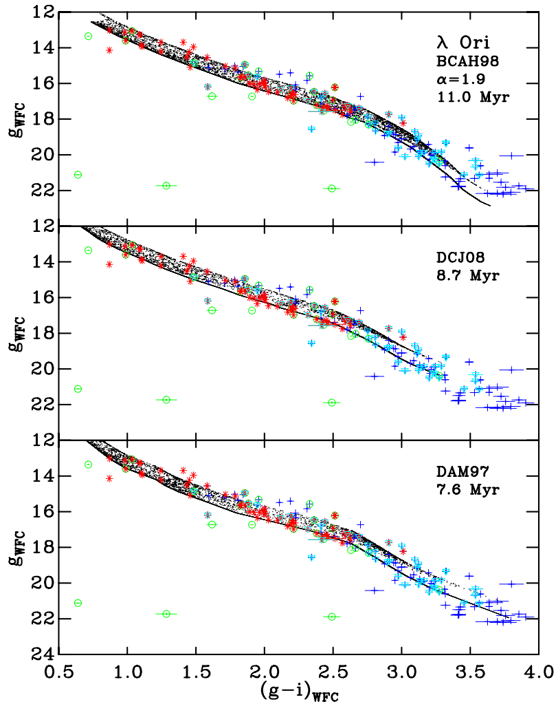
Figure 5.7: Pre-MS stars selected as members of the \lambda Ori association. Asterisks are LiI spectroscopic members from Dolan & Mathieu (2001), crosses are the combined H\alpha spectroscopic and IR excess sources from Barrado y Navascués et al. (2007), triangles are LiI and H\alpha spectroscopic members from Sacco et al. (2008), and circles are the X-ray sources from Barrado et al. (2011). Overlaid are the best-fitting isochrones of BCAH98 \alpha = 1.9 (upper panel), DCJ08 (middle panel), and DAM97 (lower panel) at the best-fit MS distance. The probability densities \rho are shown as the greyscale isochrones.
