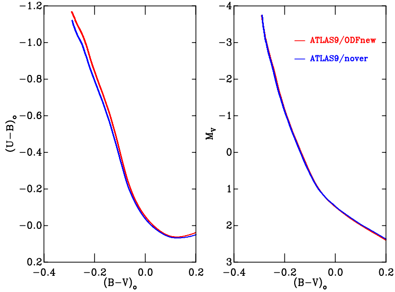
Figure 2.36: 1 Myr Geneva-Bessell isochrones. Left: Intrinsic (U - B)_\odot , (B - V)_\odot colour-colour diagram. Right: Absolute magnitude-intrinsic colour M_V , (B - V)_\odot CMD. The Schaller et al. (1992) interior models have been transformed into the observable plane using BC- T_{\text{eff}} relations based on the ATLAS9 “no-overshoot” models (Bessell et al. 1998; blue) and the updated ATLAS9/ODFnew model atmospheres as derived in this study (red). The ATLAS9/ODFnew model atmospheres result in a modified shape to the (U - B)_\odot , (B - V)_\odot isochrone for colours (B - V)_\odot \lesssim 0 . Note however that no similar effect is observed in the M_V , (B - V)_\odot CMD.
