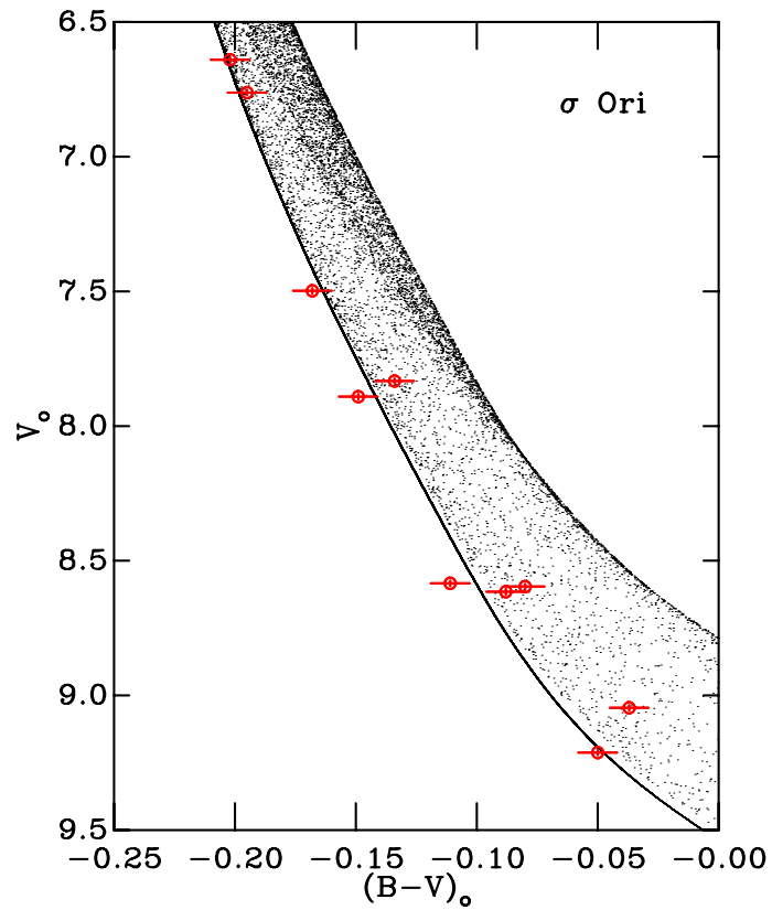
Figure 2.33: The best-fitting V_0, (B - V)_0 CMD for \sigma Ori, with an age of 8.7 Myr and distance modulus dm = 8.05 . The probability density \rho is shown as the greyscale isochrone. Circles represent the photometric data of Greenstein & Wallerstein (1958), Hardie et al. (1964), and Guetter (1979). The plotted uncertainties are the magnitude independent values discussed in Section 2.8.4.10.
