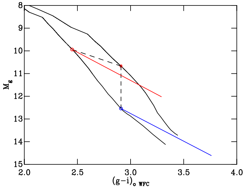
Figure 5.6: Two 5 Myr BCAH98 \alpha = 1.9 isochrones transformed into CMD space using the original BC- T_{\text{eff}} relation (lower isochrone) and the adjusted BC- T_{\text{eff}} relation (upper isochrone). The red circle represents a star of mass 0.3 M_{\odot} based on the original BC- T_{\text{eff}} relation, the red asterisk is a star of the same mass using the adjusted BC- T_{\text{eff}} relation, and the blue circle is a star of the same colour as that on the adjusted isochrone. The red and blue diagonal lines denote the reddening vectors for the red and blue circles respectively (calculated at a nominal E(B - V) = 0.5 using the interstellar extinction law of Cardelli et al. 1989).
