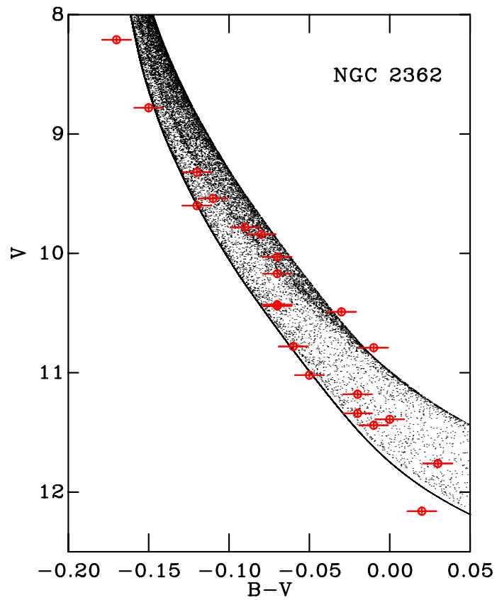
Figure 2.23: The best-fitting V, B - V CMD for NGC 2362, with an age of 12.6 Myr and distance modulus dm = 10.60 . The probability density \rho is shown as the greyscale isochrone. Circles represent the photometric data of Johnson & Morgan (1953), with the associated uncertainties shown as the bars.
