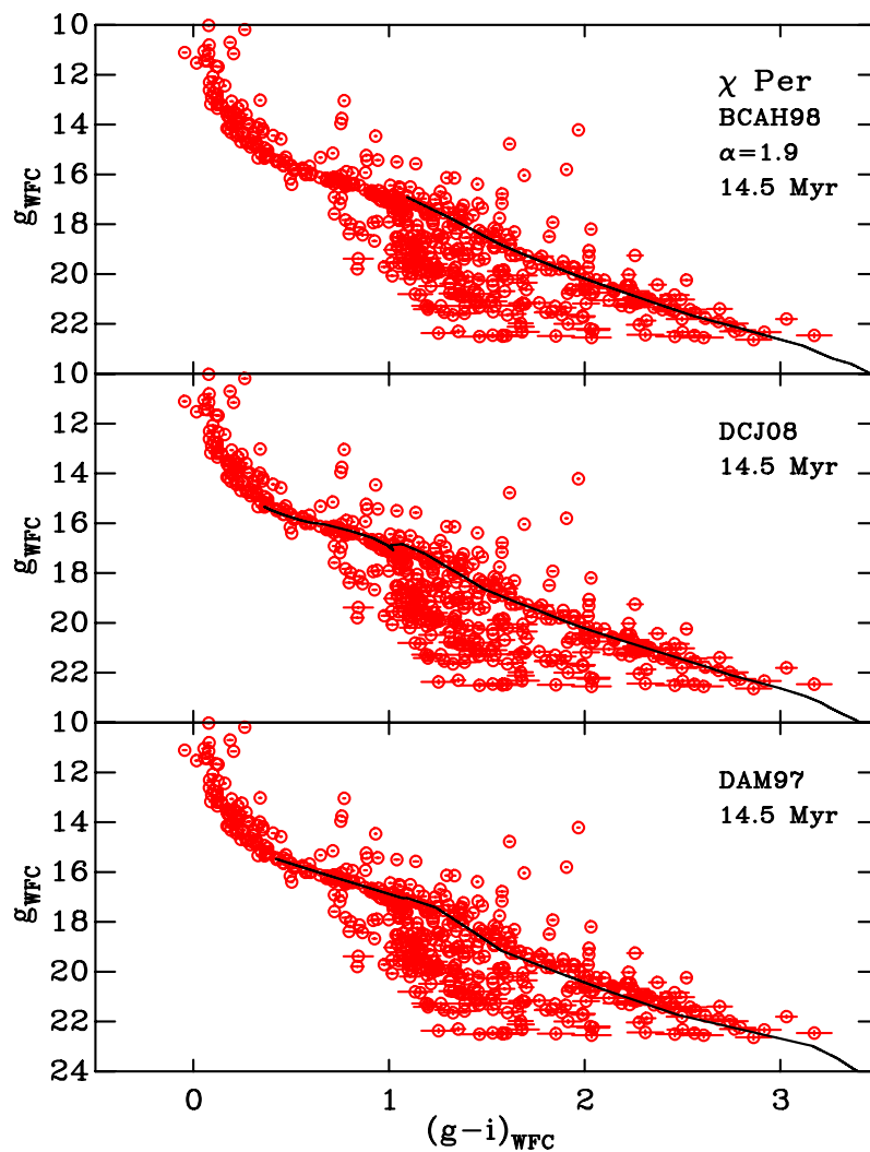
Figure 5.21: \chi Per g_{\text{WFC}}, (g-i)_{\text{WFC}} CMD with stars selected as possible members based on their positions on the sky relative to the cluster centre (see Section 5.3.2). The 14.5 Myr semi-empirical pre-MS model isochrones of BCAH98 \alpha = 1.9 , DCJ08, and DAM97 are overlaid at a distance modulus of dm = 11.8 and reddened by E(B-V) = 0.52 .
