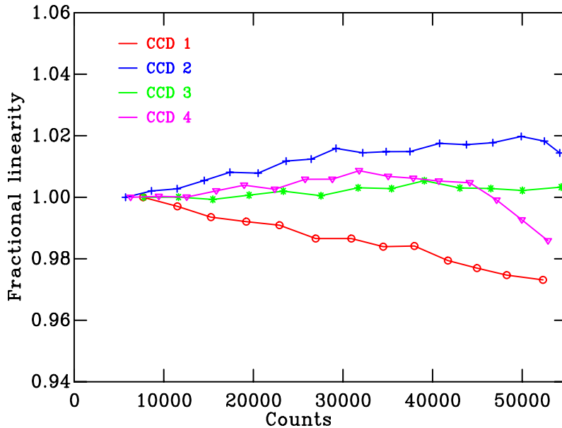
Figure 3.2: Linearity curves for the four EEV CCDs as performed in September 2008 for the “fast” readout mode on the INT-WFC.
