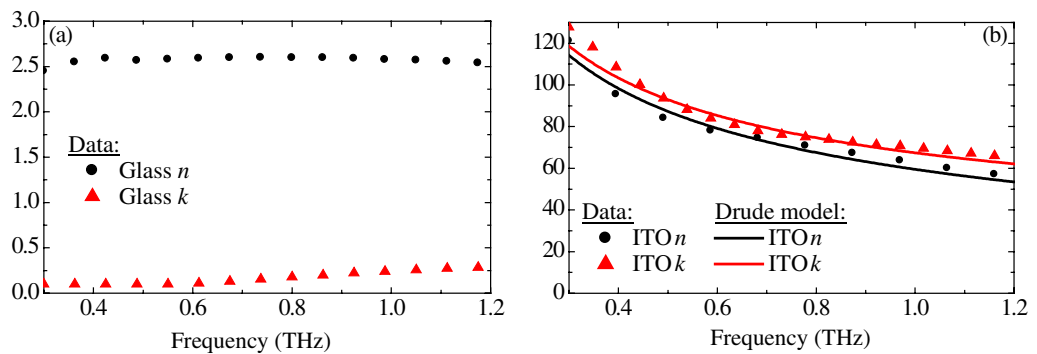
Figure 3. Measured dispersion over the spectral range used in the experiment of the refractive index and absorption of (a) glass and (b) ITO (including the results from the Drude model using the values given in the text).
