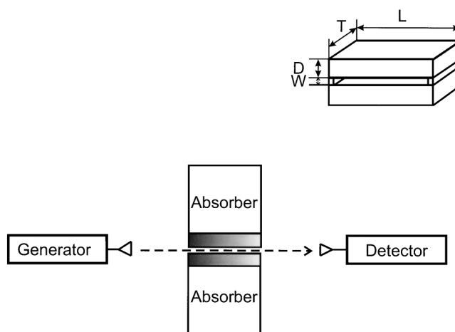
FIG. 1. The experimental setup and sample geometry.
