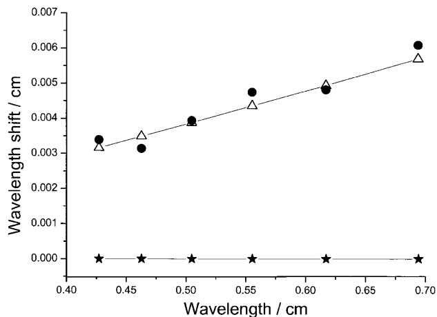
FIG. 3. Theoretical prediction ( \Delta ) and experimental data ( \bullet ) of the wavelength shifts from the simple Fabry-Pérot resonance condition.
