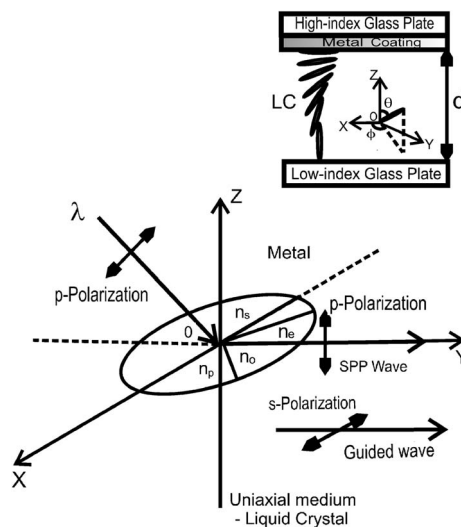
FIG. 1. The SPP mode and guided waves at the top-boundary area of a HAN-LC cell. The inset is a HLGM-HAN-LC cell with a metal tunnel barrier.
